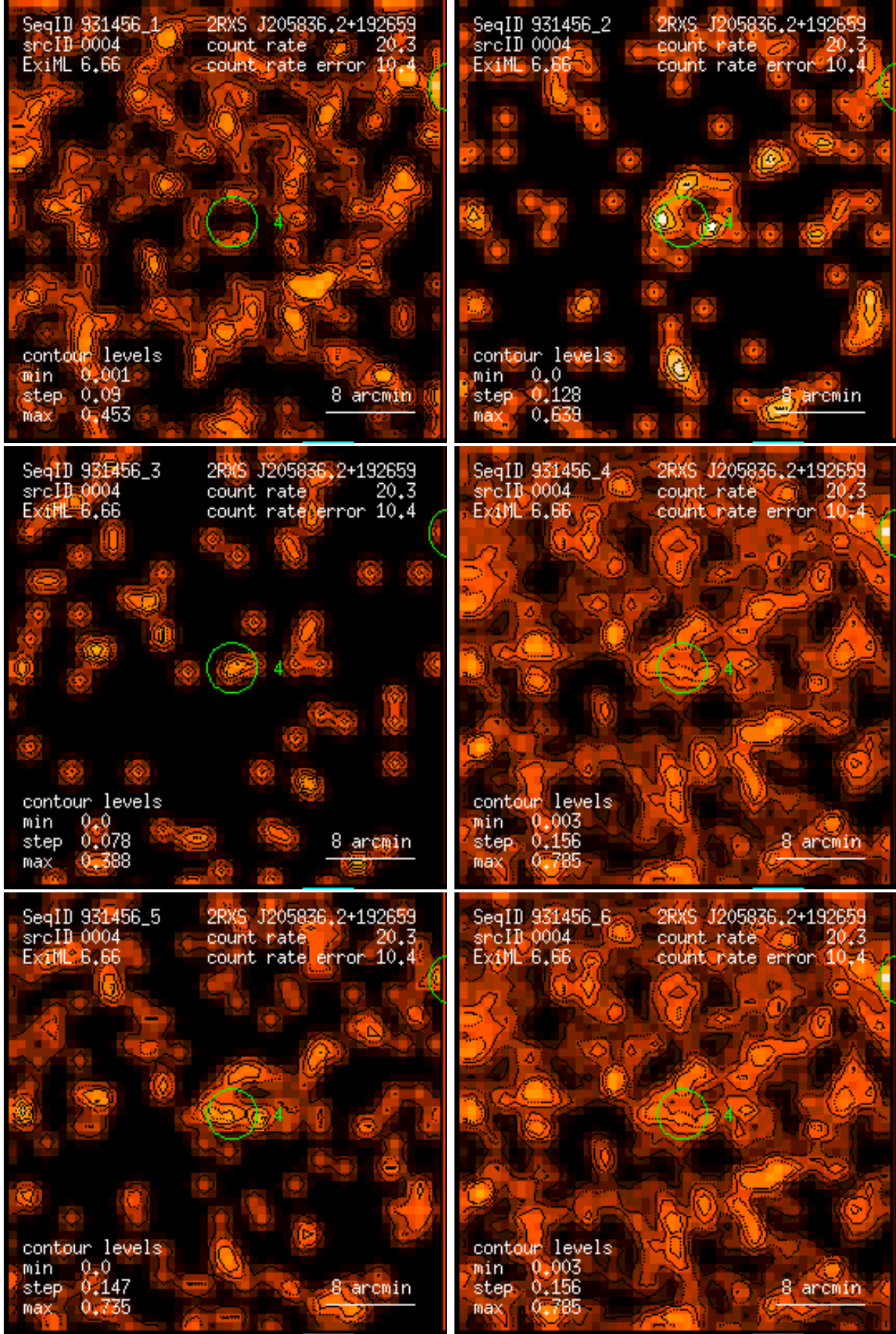
Figure 4: RASS 931456: detection 0004: band rate images, Gaussian filter: (1) PSPC channels 11 – 41, (2) 52 – 90, (3) 91 – 201, (4) 11 – 235, (5) 52 – 201, (6) 11 – 201. Broad band rates in counts/ks. Band rate contour levels in counts/ks/arcmin 2 .
