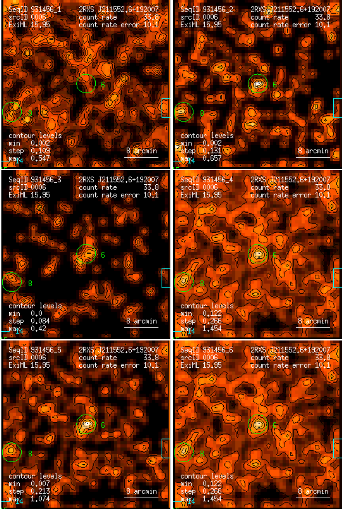
Figure 6: RASS 931456: detection 0006: band rate images, Gaussian filter: (1) PSPC channels 11 – 41, (2) 52 – 90, (3) 91 – 201, (4) 11 – 235, (5) 52 – 201, (6) 11 – 201. Broad band rates in counts/ks. Band rate contour levels in counts/ks/arcmin 2 .
