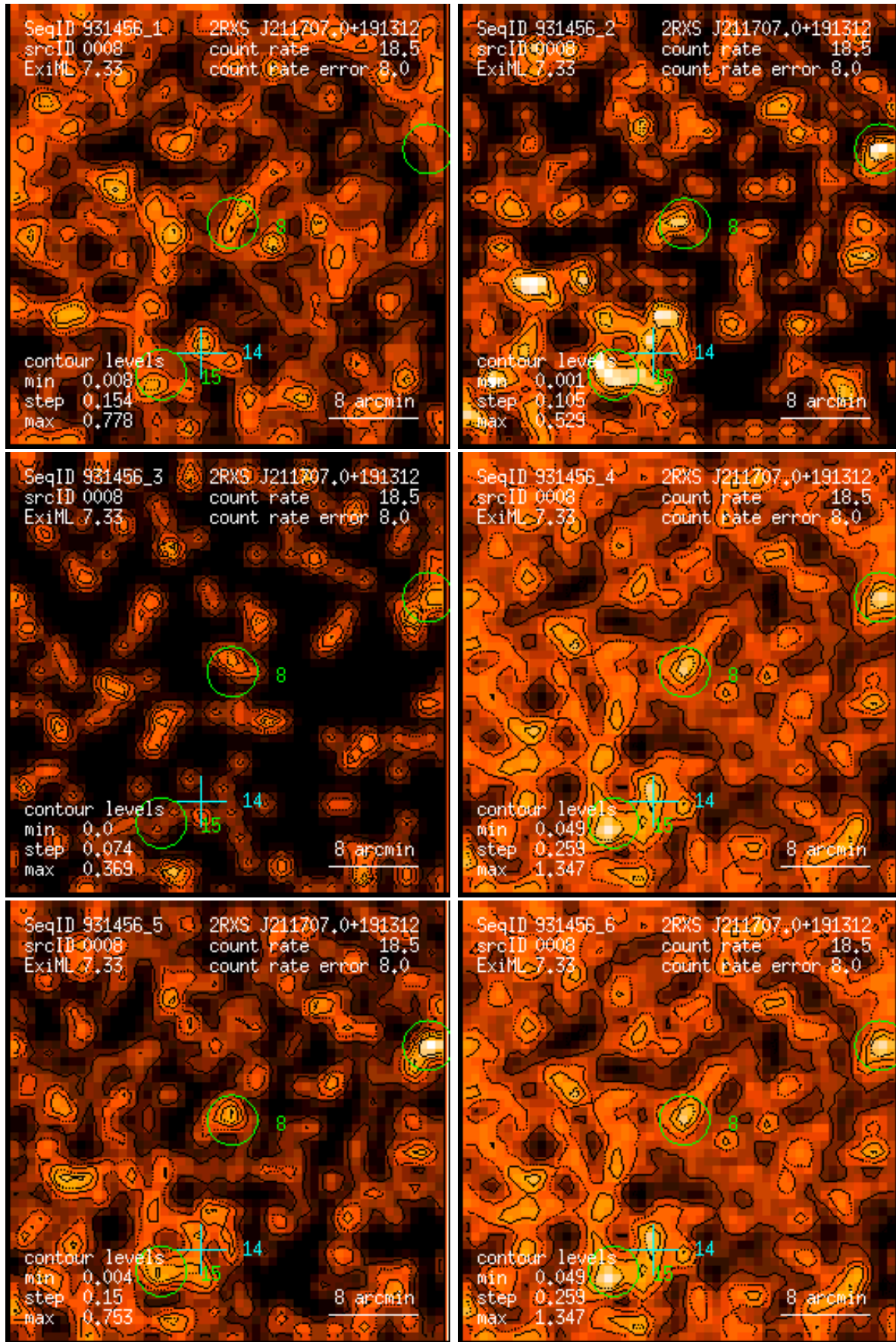
Figure 8: RASS 931456: detection 0008: band rate images, Gaussian filter: (1) PSPC channels 11 – 41, (2) 52 – 90, (3) 91 – 201, (4) 11 – 235, (5) 52 – 201, (6) 11 – 201. Broad band rates in counts/ks. Band rate contour levels in counts/ks/arcmin 2 .
