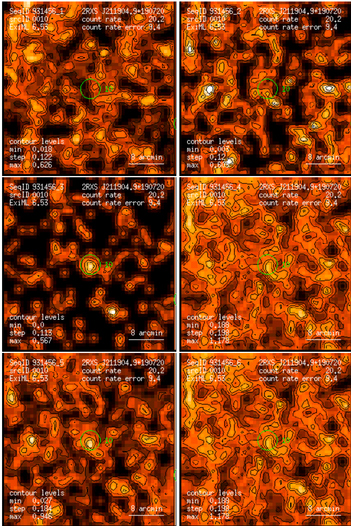
Figure 10: RASS 931456: detection 0010: band rate images, Gaussian filter: (1) PSPC channels 11 – 41, (2) 52 – 90, (3) 91 – 201, (4) 11 – 235, (5) 52 – 201, (6) 11 – 201. Broad band rates in counts/ks. Band rate contour levels in counts/ks/arcmin 2 .
