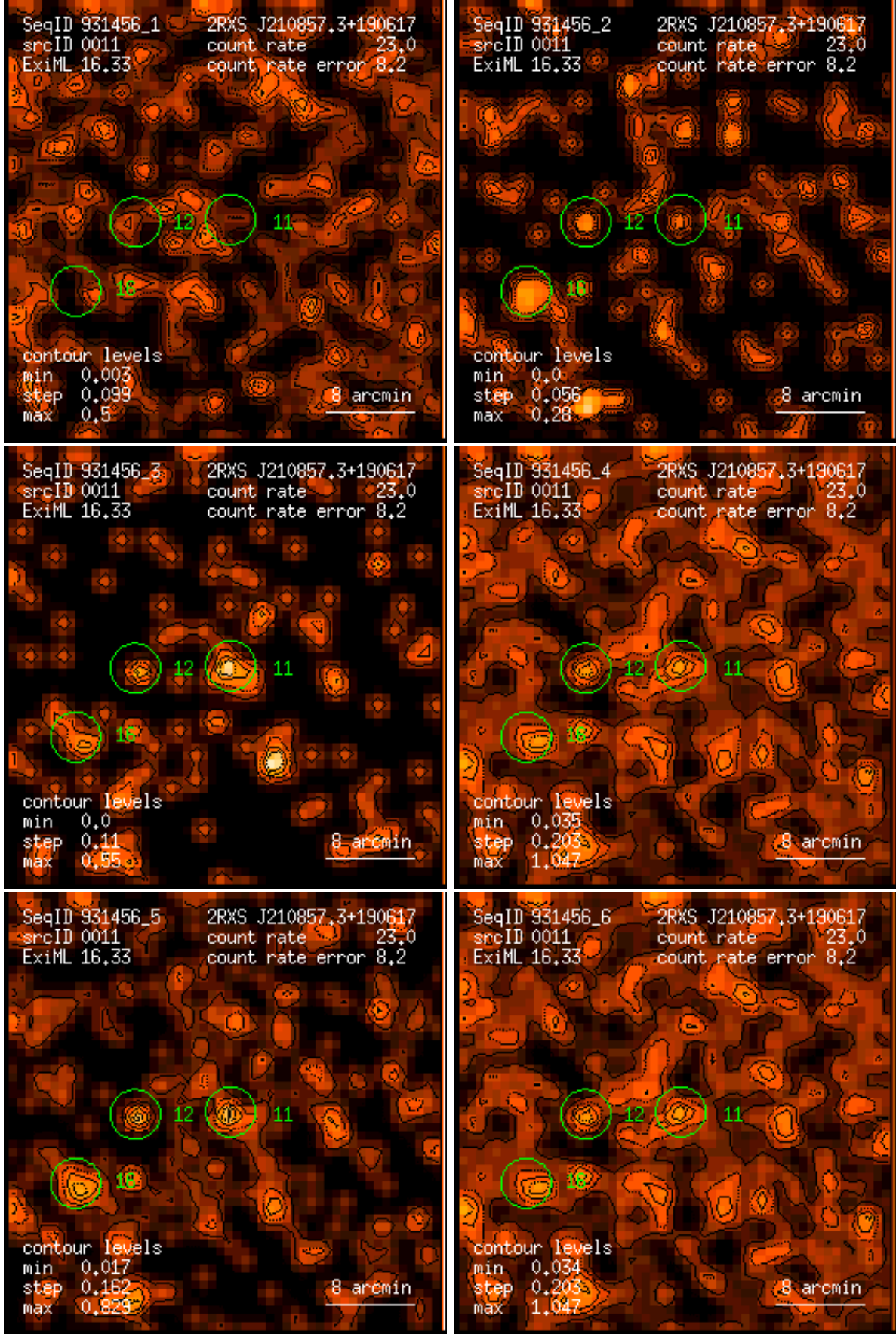
Figure 11: RASS 931456: detection 0011: band rate images, Gaussian filter: (1) PSPC channels 11 – 41, (2) 52 – 90, (3) 91 – 201, (4) 11 – 235, (5) 52 – 201, (6) 11 – 201. Broad band rates in counts/ks. Band rate contour levels in counts/ks/arcmin 2 .
