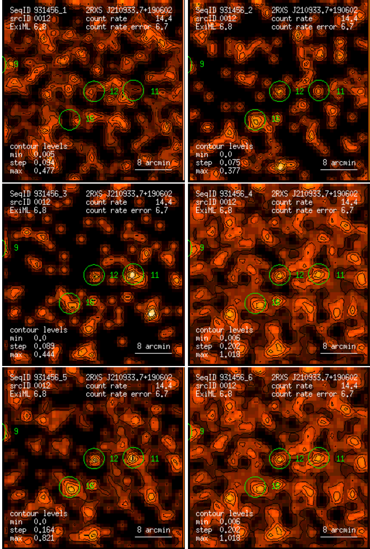
Figure 12: RASS 931456: detection 0012: band rate images, Gaussian filter: (1) PSPC channels 11 – 41, (2) 52 – 90, (3) 91 – 201, (4) 11 – 235, (5) 52 – 201, (6) 11 – 201. Broad band rates in counts/ks. Band rate contour levels in counts/ks/arcmin 2 .
