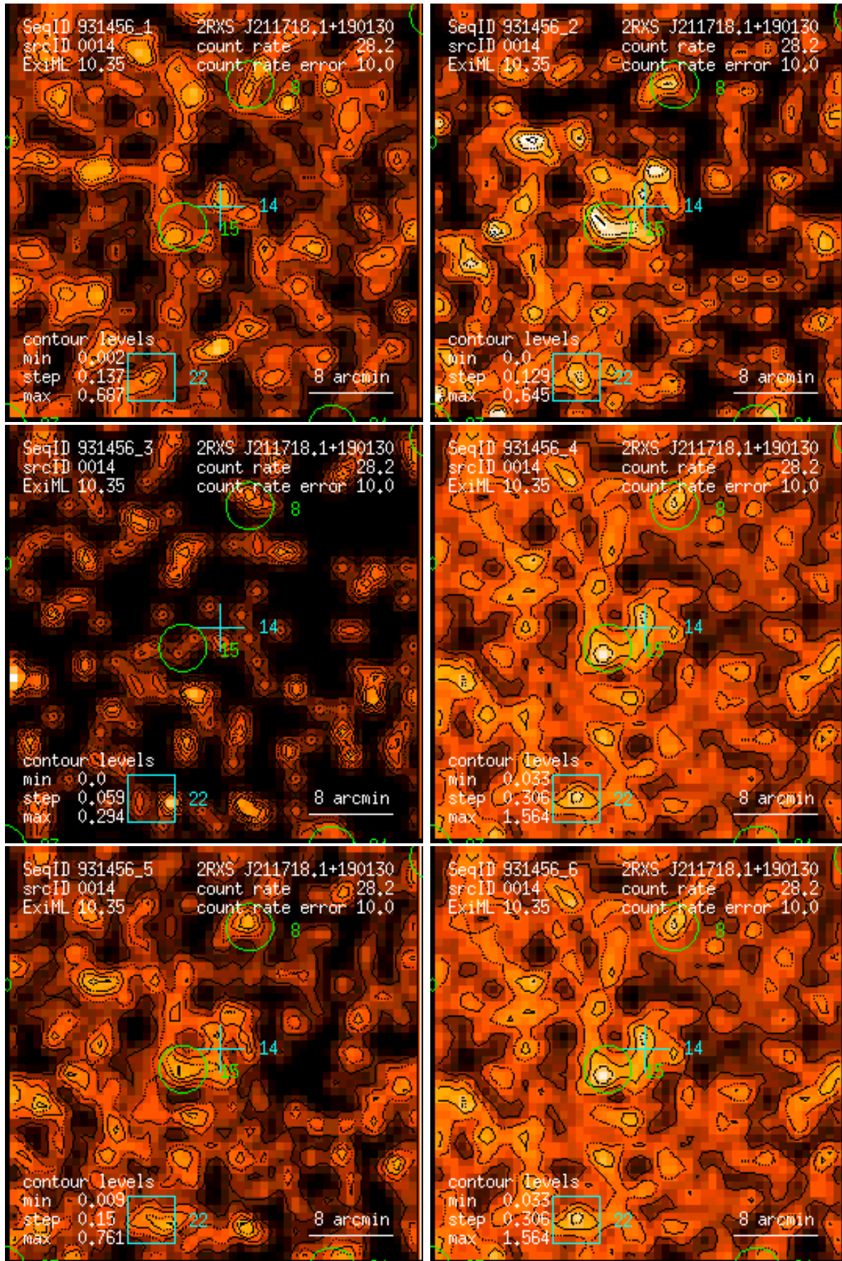
Figure 14: RASS 931456: detection 0014: band rate images, Gaussian filter: (1) PSPC channels 11 – 41, (2) 52 – 90, (3) 91 – 201, (4) 11 – 235, (5) 52 – 201, (6) 11 – 201. Broad band rates in counts/ks. Band rate contour levels in counts/ks/arcmin 2 .
