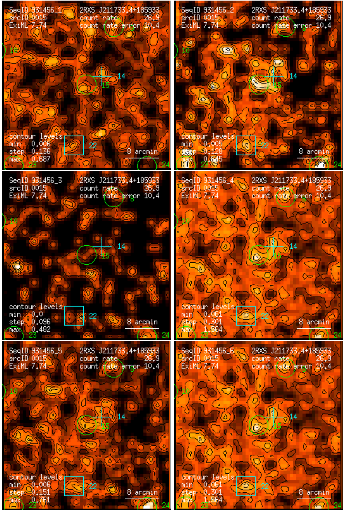
Figure 15: RASS 931456: detection 0015: band rate images, Gaussian filter: (1) PSPC channels 11 – 41, (2) 52 – 90, (3) 91 – 201, (4) 11 – 235, (5) 52 – 201, (6) 11 – 201. Broad band rates in counts/ks. Band rate contour levels in counts/ks/arcmin 2 .
