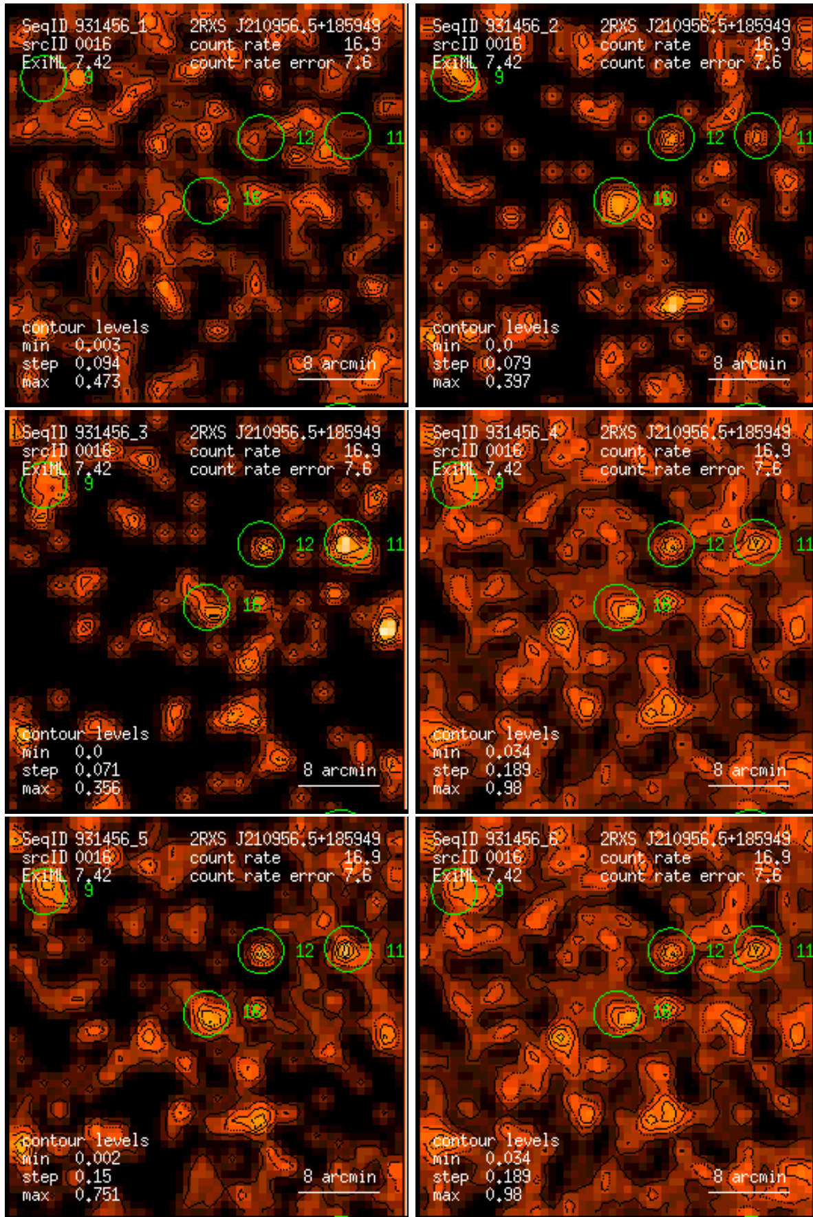
Figure 16: RASS 931456: detection 0016: band rate images, Gaussian filter: (1) PSPC channels 11 – 41, (2) 52 – 90, (3) 91 – 201, (4) 11 – 235, (5) 52 – 201, (6) 11 – 201. Broad band rates in counts/ks. Band rate contour levels in counts/ks/arcmin 2 .
