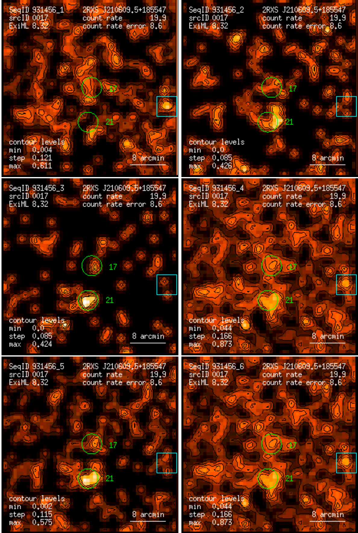
Figure 17: RASS 931456: detection 0017: band rate images, Gaussian filter: (1) PSPC channels 11 – 41, (2) 52 – 90, (3) 91 – 201, (4) 11 – 235, (5) 52 – 201, (6) 11 – 201. Broad band rates in counts/ks. Band rate contour levels in counts/ks/arcmin 2 .
