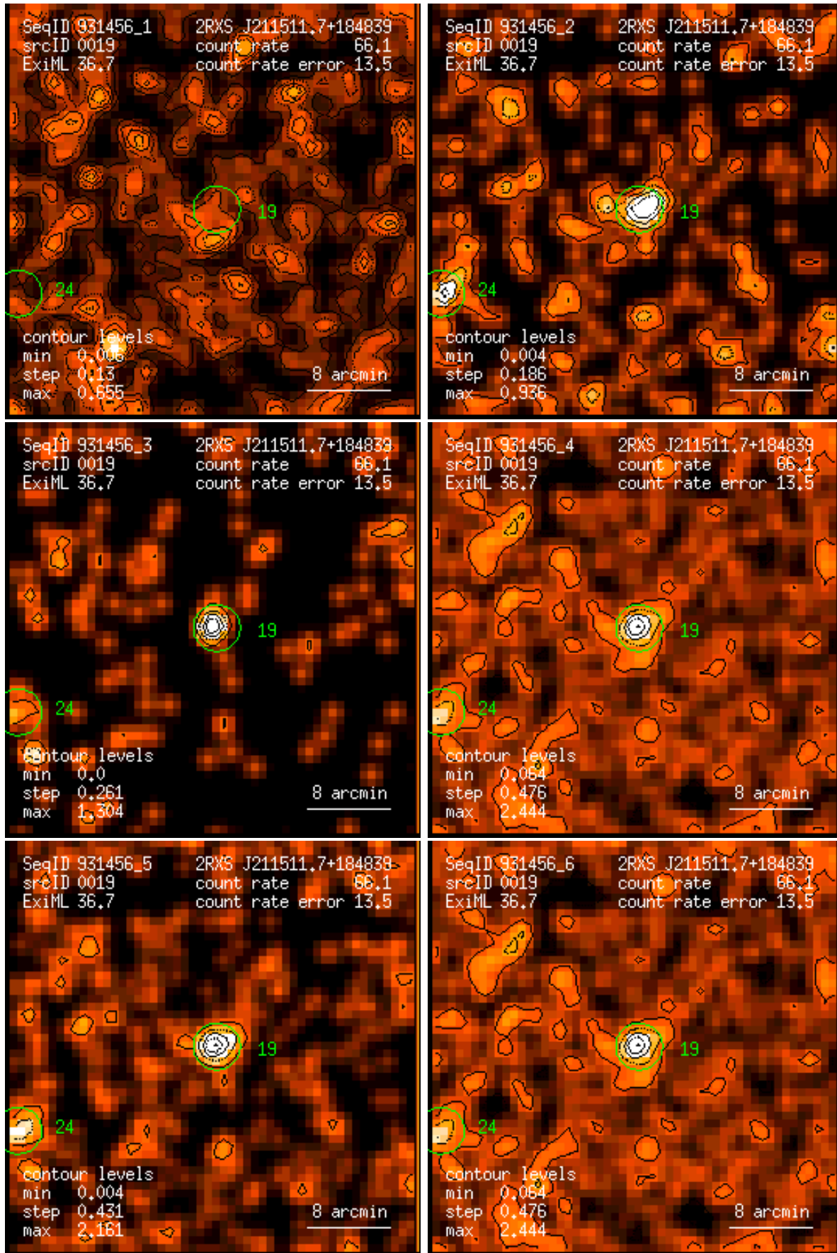
Figure 19: RASS 931456: detection 0019: band rate images, Gaussian filter: (1) PSPC channels 11 – 41, (2) 52 – 90, (3) 91 – 201, (4) 11 – 235, (5) 52 – 201, (6) 11 – 201. Broad band rates in counts/ks. Band rate contour levels in counts/ks/arcmin 2 .
