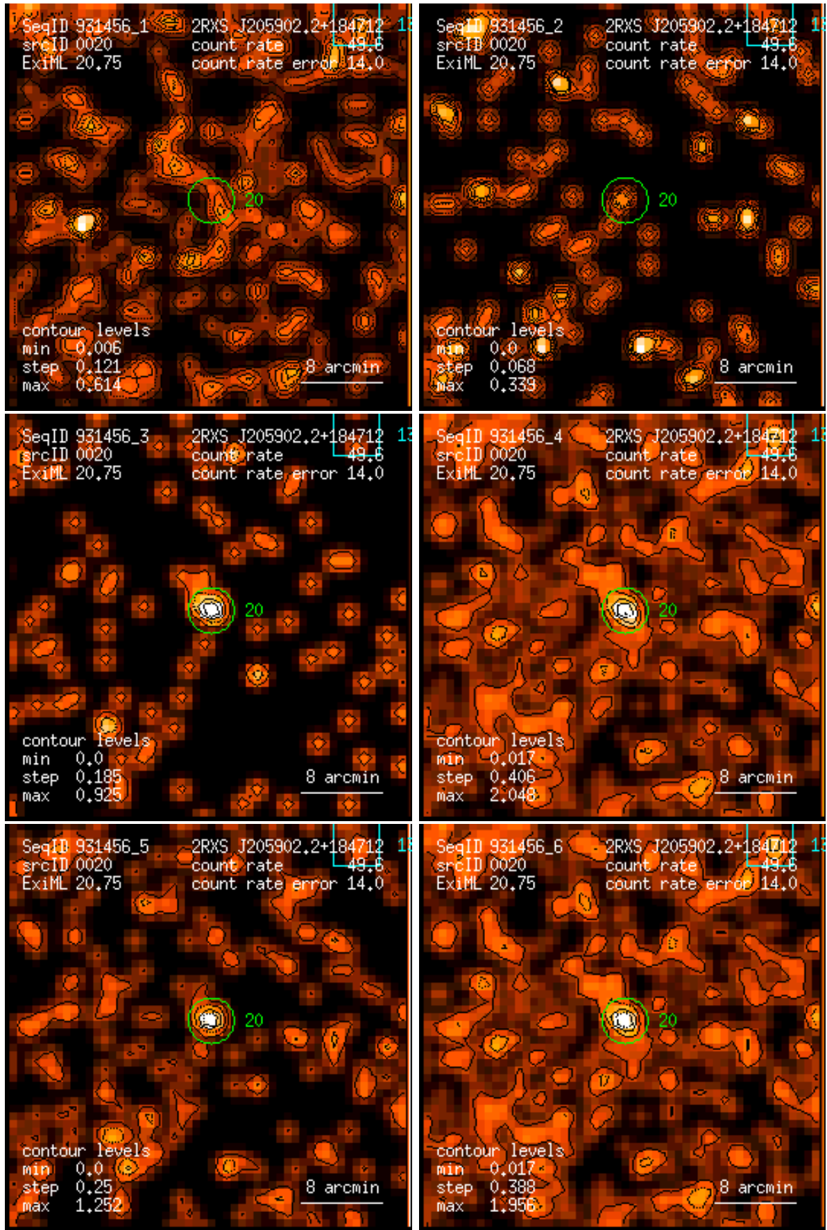
Figure 20: RASS 931456: detection 0020: band rate images, Gaussian filter: (1) PSPC channels 11 – 41, (2) 52 – 90, (3) 91 – 201, (4) 11 – 235, (5) 52 – 201, (6) 11 – 201. Broad band rates in counts/ks. Band rate contour levels in counts/ks/arcmin 2 .
