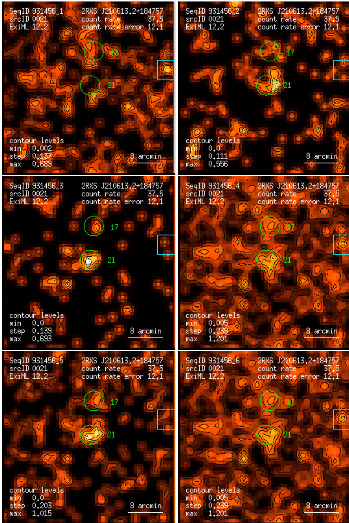
Figure 21: RASS 931456: detection 0021: band rate images, Gaussian filter: (1) PSPC channels 11 – 41, (2) 52 – 90, (3) 91 – 201, (4) 11 – 235, (5) 52 – 201, (6) 11 – 201. Broad band rates in counts/ks. Band rate contour levels in counts/ks/arcmin 2 .
