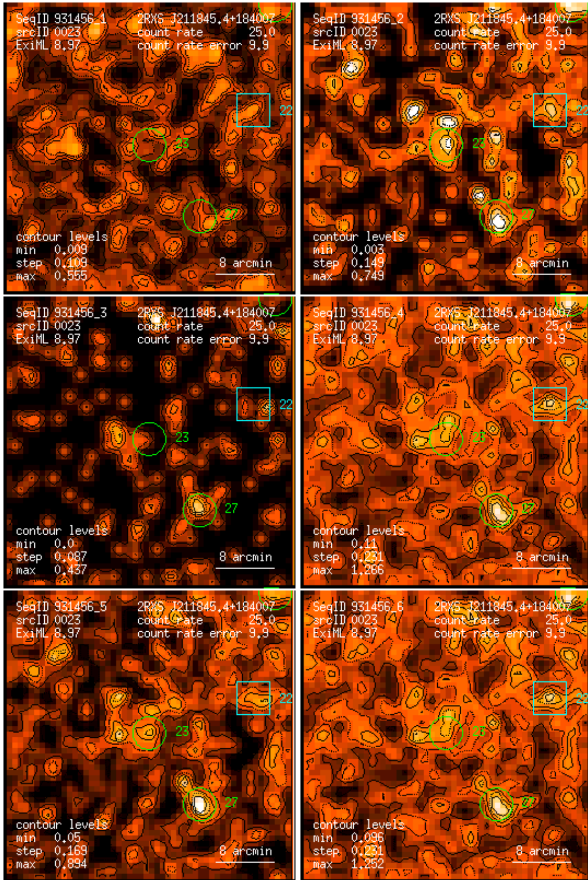
Figure 23: RASS 931456: detection 0023: band rate images, Gaussian filter: (1) PSPC channels 11 – 41, (2) 52 – 90, (3) 91 – 201, (4) 11 – 235, (5) 52 – 201, (6) 11 – 201. Broad band rates in counts/ks. Band rate contour levels in counts/ks/arcmin 2 .
