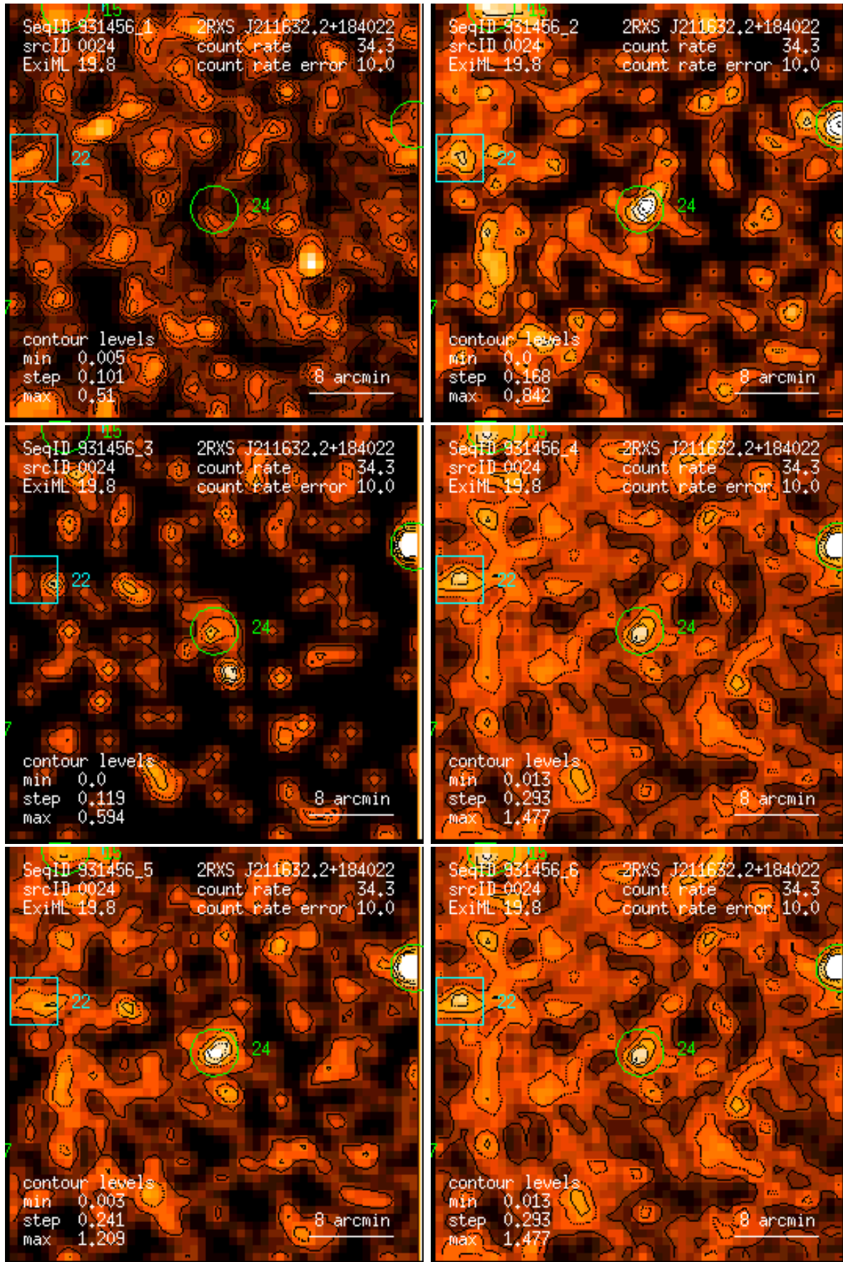
Figure 24: RASS 931456: detection 0024: band rate images, Gaussian filter: (1) PSPC channels 11 – 41, (2) 52 – 90, (3) 91 – 201, (4) 11 – 235, (5) 52 – 201, (6) 11 – 201. Broad band rates in counts/ks. Band rate contour levels in counts/ks/arcmin 2 .
