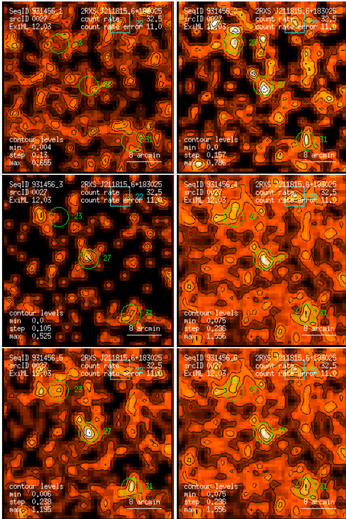
Figure 27: RASS 931456: detection 0027: band rate images, Gaussian filter: (1) PSPC channels 11 – 41, (2) 52 – 90, (3) 91 – 201, (4) 11 – 235, (5) 52 – 201, (6) 11 – 201. Broad band rates in counts/ks. Band rate contour levels in counts/ks/arcmin 2 .
