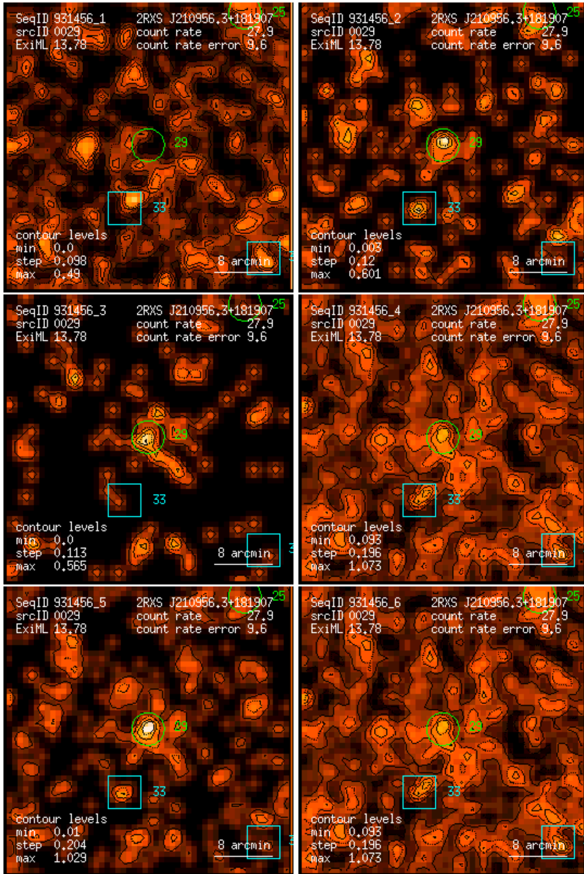
Figure 29: RASS 931456: detection 0029: band rate images, Gaussian filter: (1) PSPC channels 11 – 41, (2) 52 – 90, (3) 91 – 201, (4) 11 – 235, (5) 52 – 201, (6) 11 – 201. Broad band rates in counts/ks. Band rate contour levels in counts/ks/arcmin 2 .
