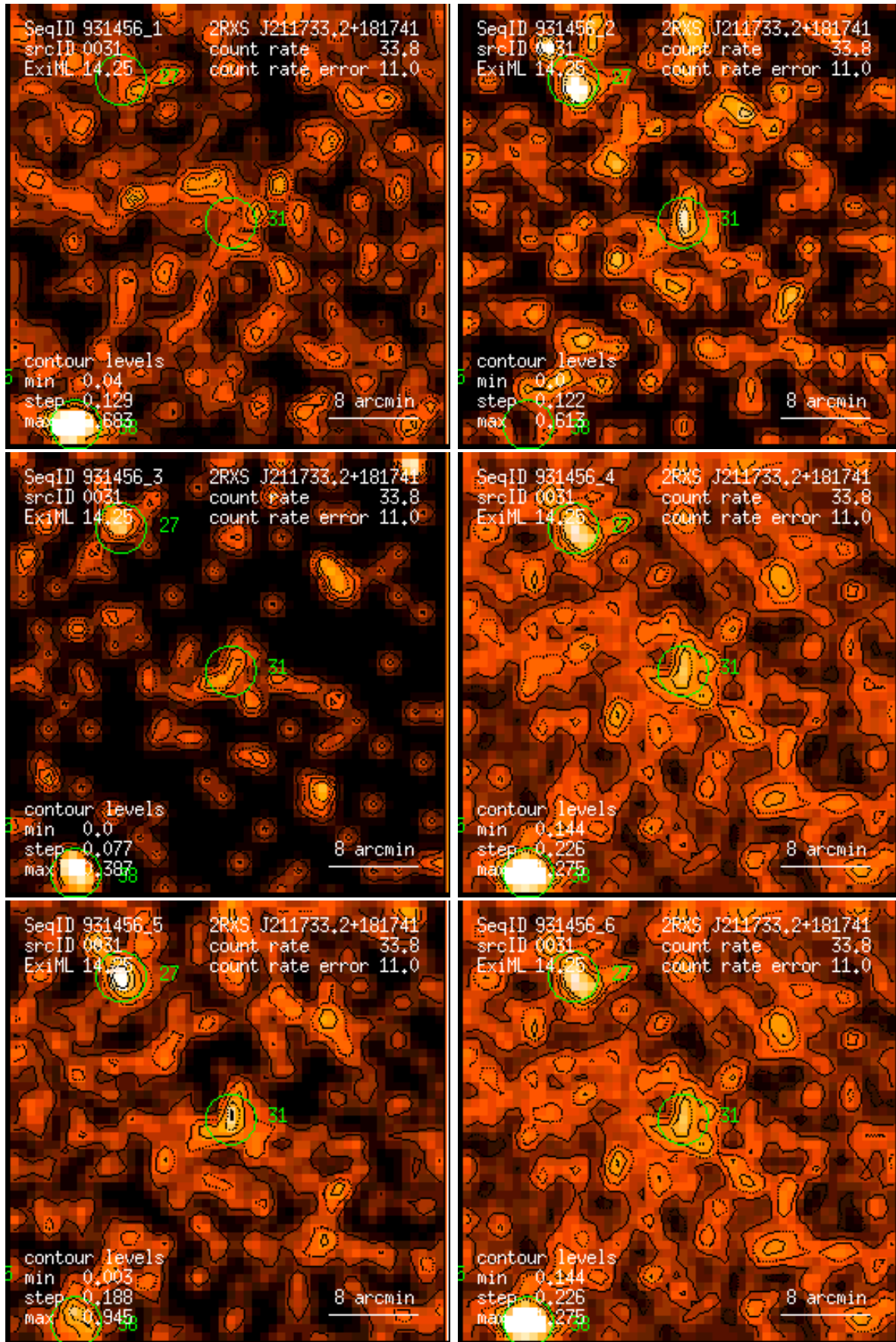
Figure 31: RASS 931456: detection 0031: band rate images, Gaussian filter: (1) PSPC channels 11 – 41, (2) 52 – 90, (3) 91 – 201, (4) 11 – 235, (5) 52 – 201, (6) 11 – 201. Broad band rates in counts/ks. Band rate contour levels in counts/ks/arcmin 2 .
