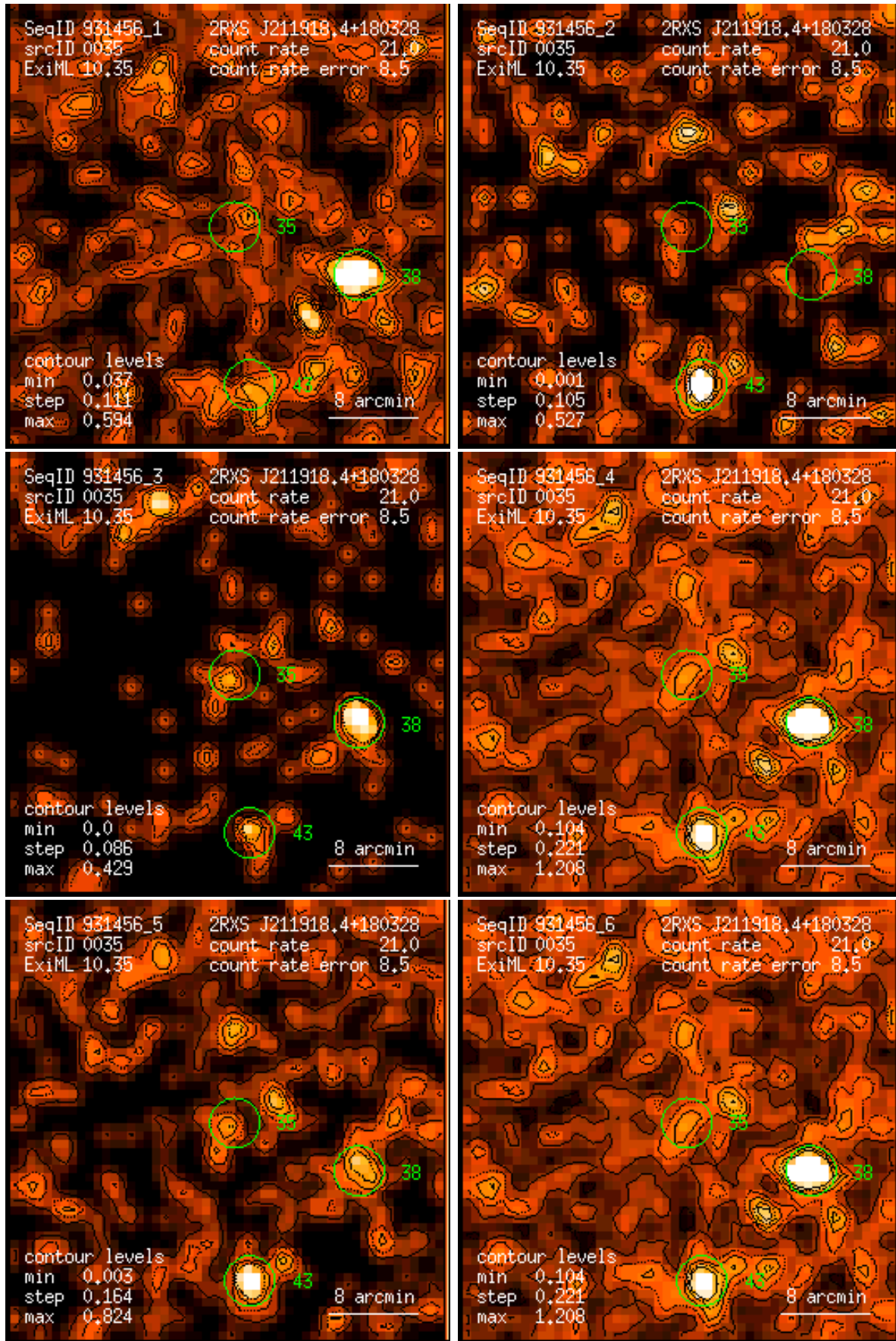
Figure 35: RASS 931456: detection 0035: band rate images, Gaussian filter: (1) PSPC channels 11 – 41, (2) 52 – 90, (3) 91 – 201, (4) 11 – 235, (5) 52 – 201, (6) 11 – 201. Broad band rates in counts/ks. Band rate contour levels in counts/ks/arcmin 2 .
