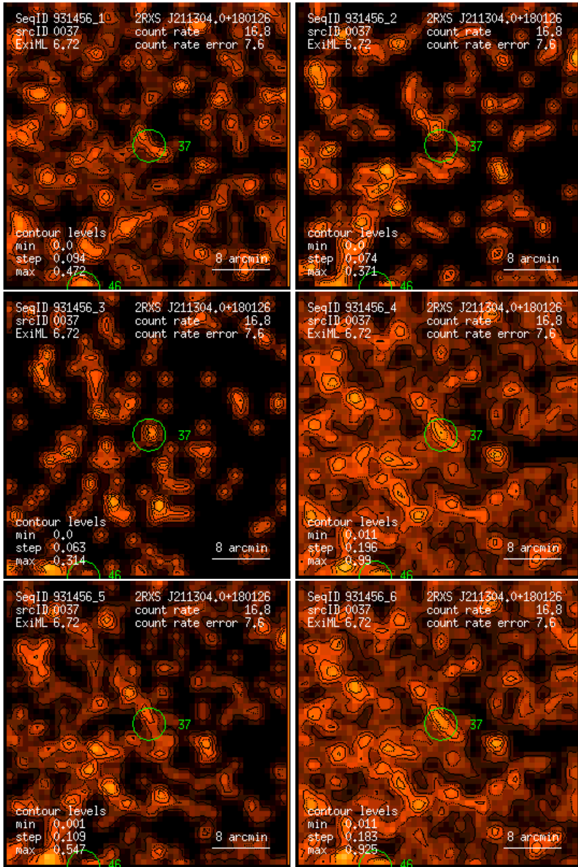
Figure 37: RASS 931456: detection 0037: band rate images, Gaussian filter: (1) PSPC channels 11 – 41, (2) 52 – 90, (3) 91 – 201, (4) 11 – 235, (5) 52 – 201, (6) 11 – 201. Broad band rates in counts/ks. Band rate contour levels in counts/ks/arcmin 2 .
