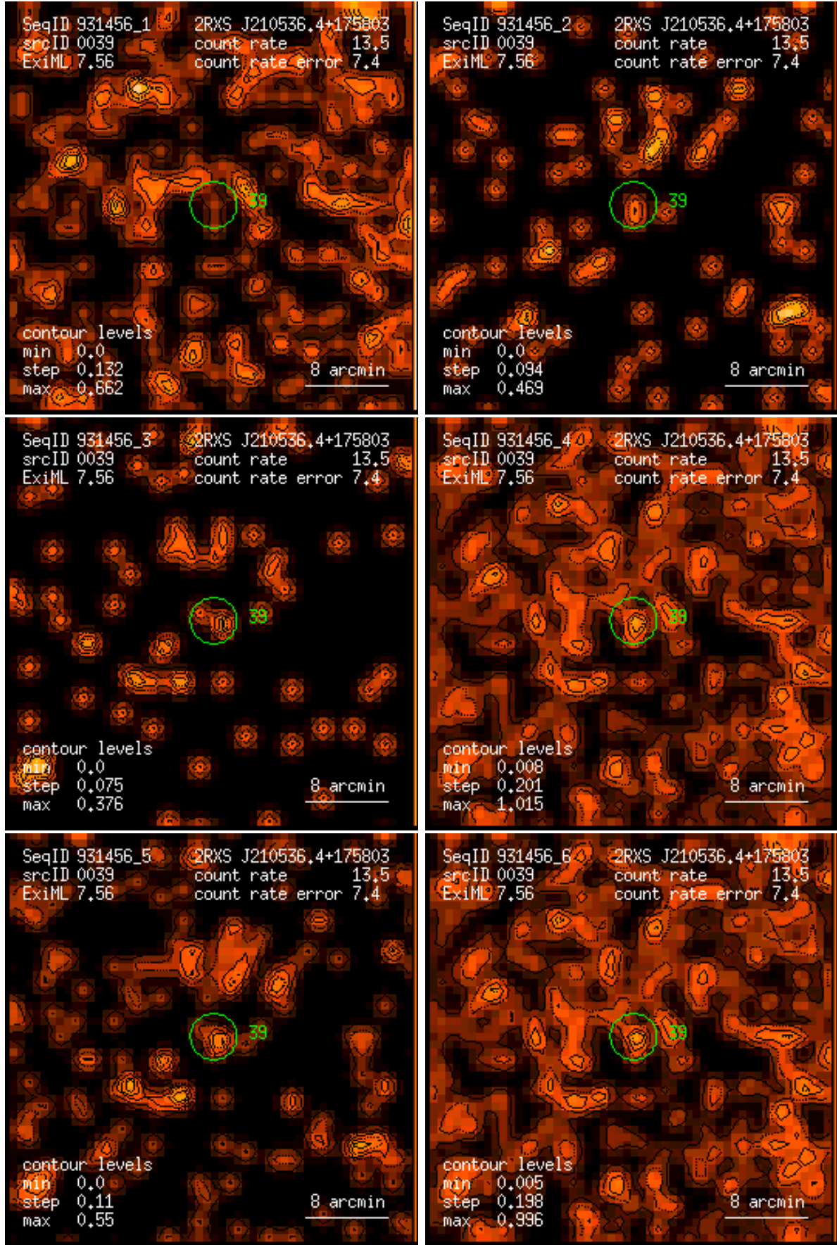
Figure 39: RASS 931456: detection 0039: band rate images, Gaussian filter: (1) PSPC channels 11 – 41, (2) 52 – 90, (3) 91 – 201, (4) 11 – 235, (5) 52 – 201, (6) 11 – 201. Broad band rates in counts/ks. Band rate contour levels in counts/ks/arcmin 2 .
