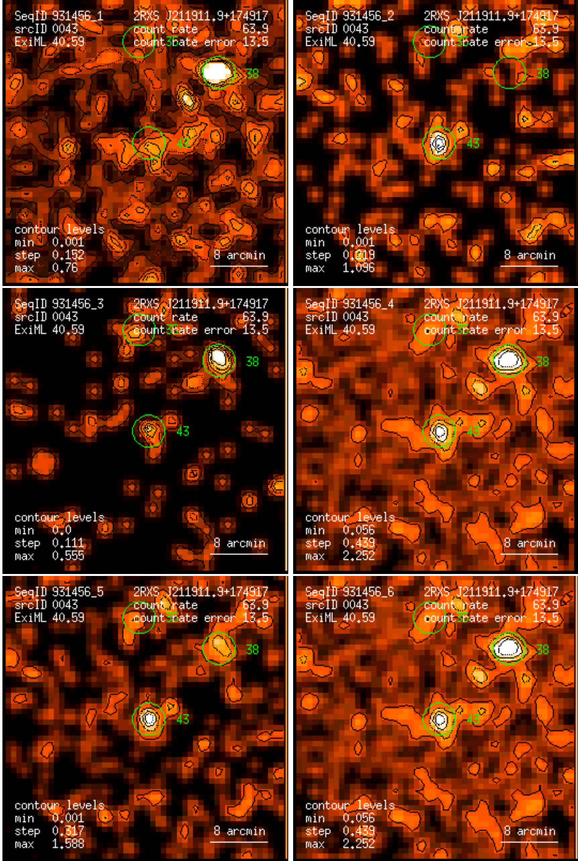
Figure 43: RASS 931456: detection 0043: band rate images, Gaussian filter: (1) PSPC channels 11 – 41, (2) 52 – 90, (3) 91 – 201, (4) 11 – 235, (5) 52 – 201, (6) 11 – 201. Broad band rates in counts/ks. Band rate contour levels in counts/ks/arcmin 2 .
