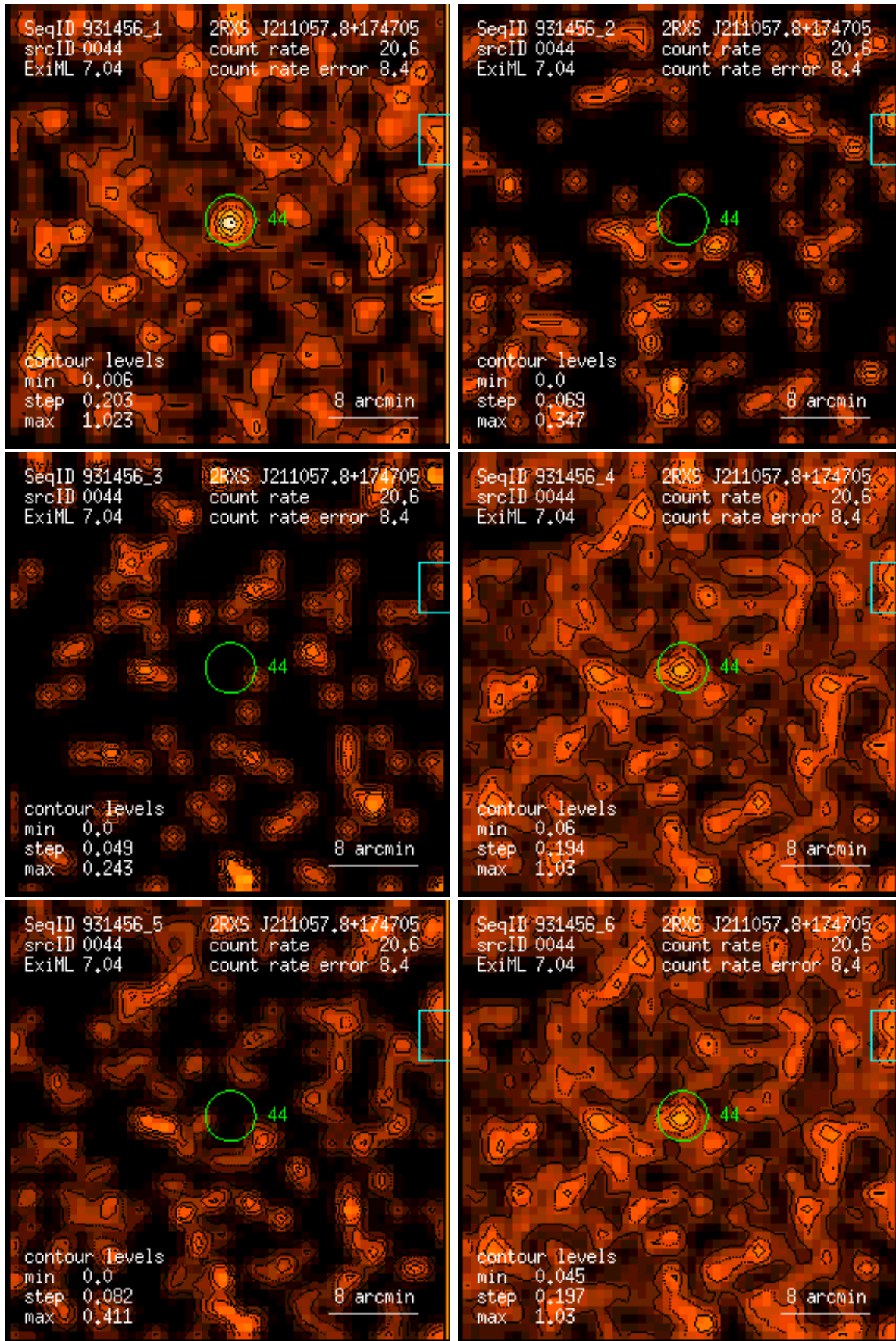
Figure 44: RASS 931456: detection 0044: band rate images, Gaussian filter: (1) PSPC channels 11 – 41, (2) 52 – 90, (3) 91 – 201, (4) 11 – 235, (5) 52 – 201, (6) 11 – 201. Broad band rates in counts/ks. Band rate contour levels in counts/ks/arcmin 2 .
