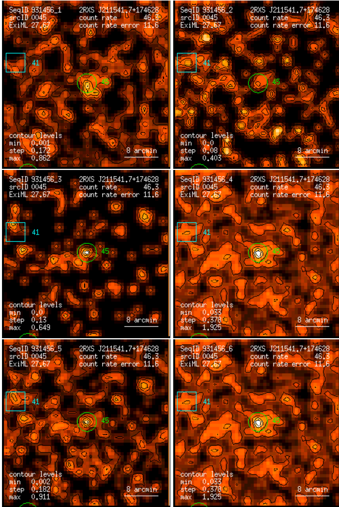
Figure 45: RASS 931456: detection 0045: band rate images, Gaussian filter: (1) PSPC channels 11 – 41, (2) 52 – 90, (3) 91 – 201, (4) 11 – 235, (5) 52 – 201, (6) 11 – 201. Broad band rates in counts/ks. Band rate contour levels in counts/ks/arcmin 2 .
