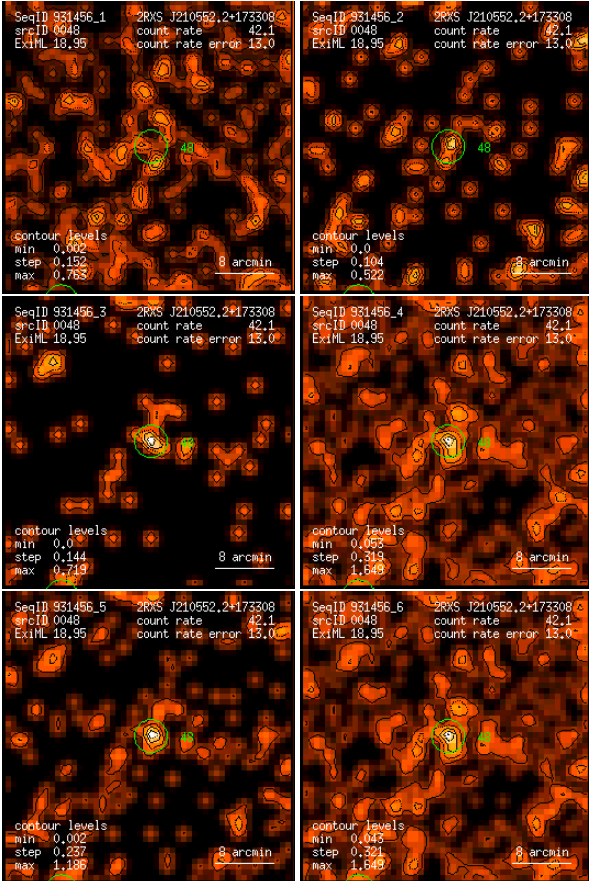
Figure 48: RASS 931456: detection 0048: band rate images, Gaussian filter: (1) PSPC channels 11 – 41, (2) 52 – 90, (3) 91 – 201, (4) 11 – 235, (5) 52 – 201, (6) 11 – 201. Broad band rates in counts/ks. Band rate contour levels in counts/ks/arcmin 2 .
