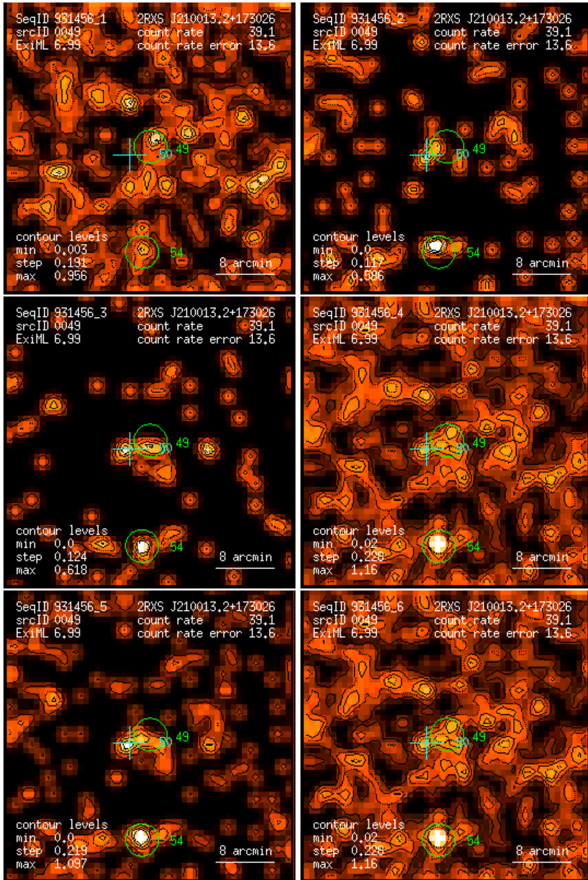
Figure 49: RASS 931456: detection 0049: band rate images, Gaussian filter: (1) PSPC channels 11 – 41, (2) 52 – 90, (3) 91 – 201, (4) 11 – 235, (5) 52 – 201, (6) 11 – 201. Broad band rates in counts/ks. Band rate contour levels in counts/ks/arcmin 2 .
