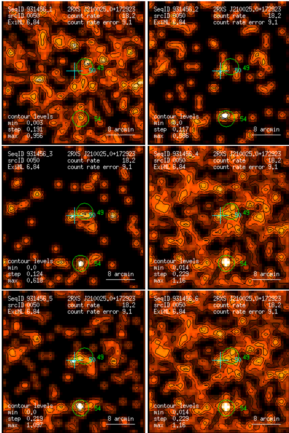
Figure 50: RASS 931456: detection 0050: band rate images, Gaussian filter: (1) PSPC channels 11 – 41, (2) 52 – 90, (3) 91 – 201, (4) 11 – 235, (5) 52 – 201, (6) 11 – 201. Broad band rates in counts/ks. Band rate contour levels in counts/ks/arcmin 2 .
