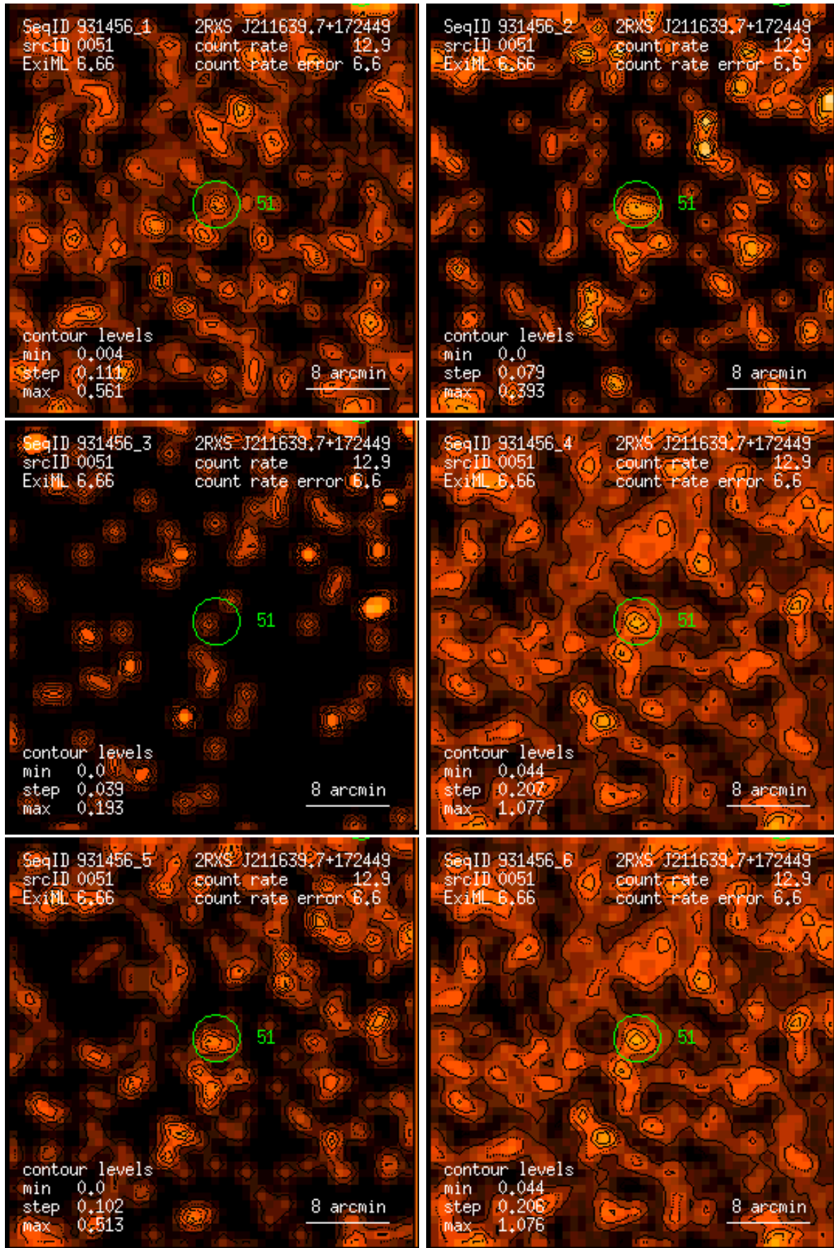
Figure 51: RASS 931456: detection 0051: band rate images, Gaussian filter: (1) PSPC channels 11 – 41, (2) 52 – 90, (3) 91 – 201, (4) 11 – 235, (5) 52 – 201, (6) 11 – 201. Broad band rates in counts/ks. Band rate contour levels in counts/ks/arcmin 2 .
