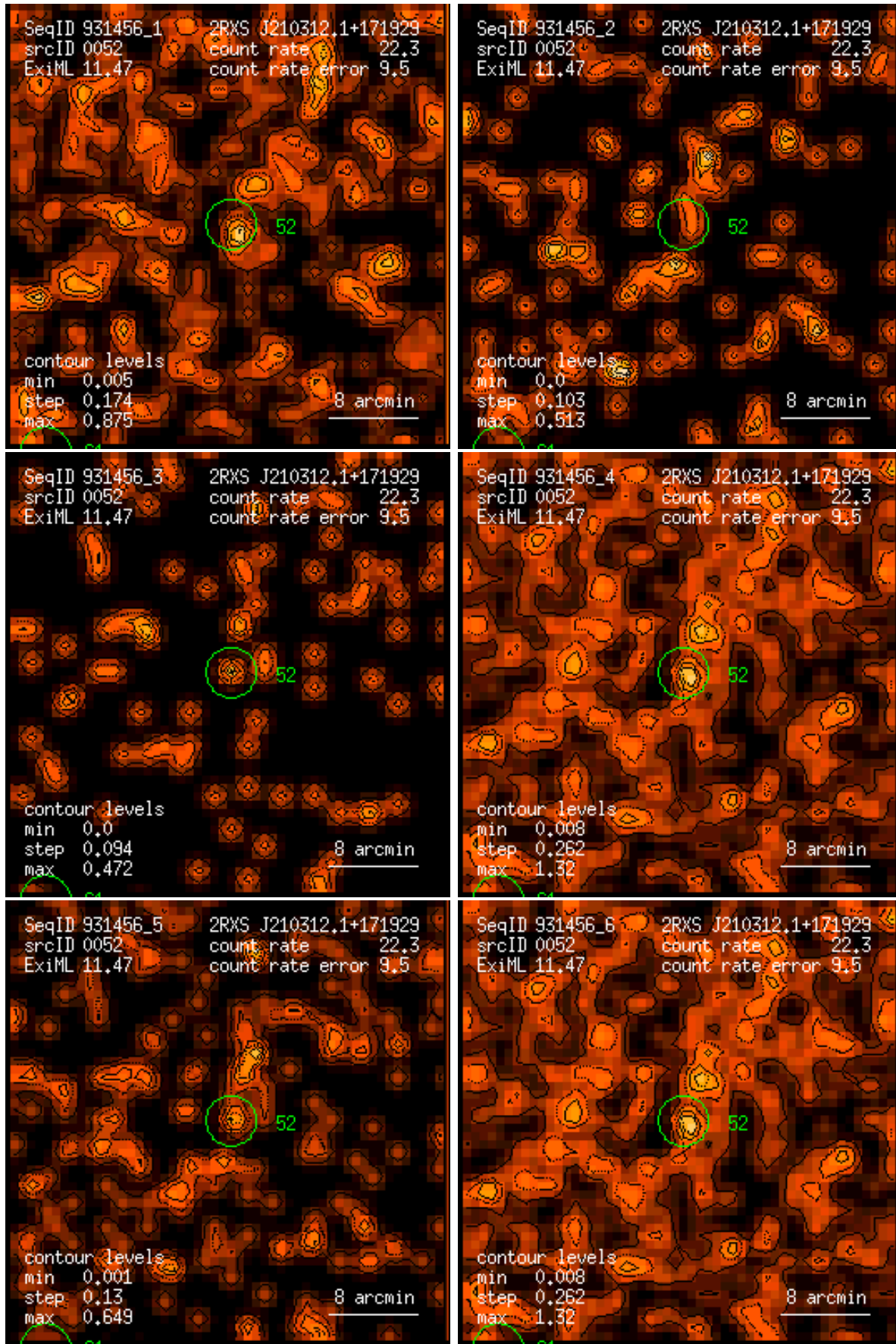
Figure 52: RASS 931456: detection 0052: band rate images, Gaussian filter: (1) PSPC channels 11 – 41, (2) 52 – 90, (3) 91 – 201, (4) 11 – 235, (5) 52 – 201, (6) 11 – 201. Broad band rates in counts/ks. Band rate contour levels in counts/ks/arcmin 2 .
