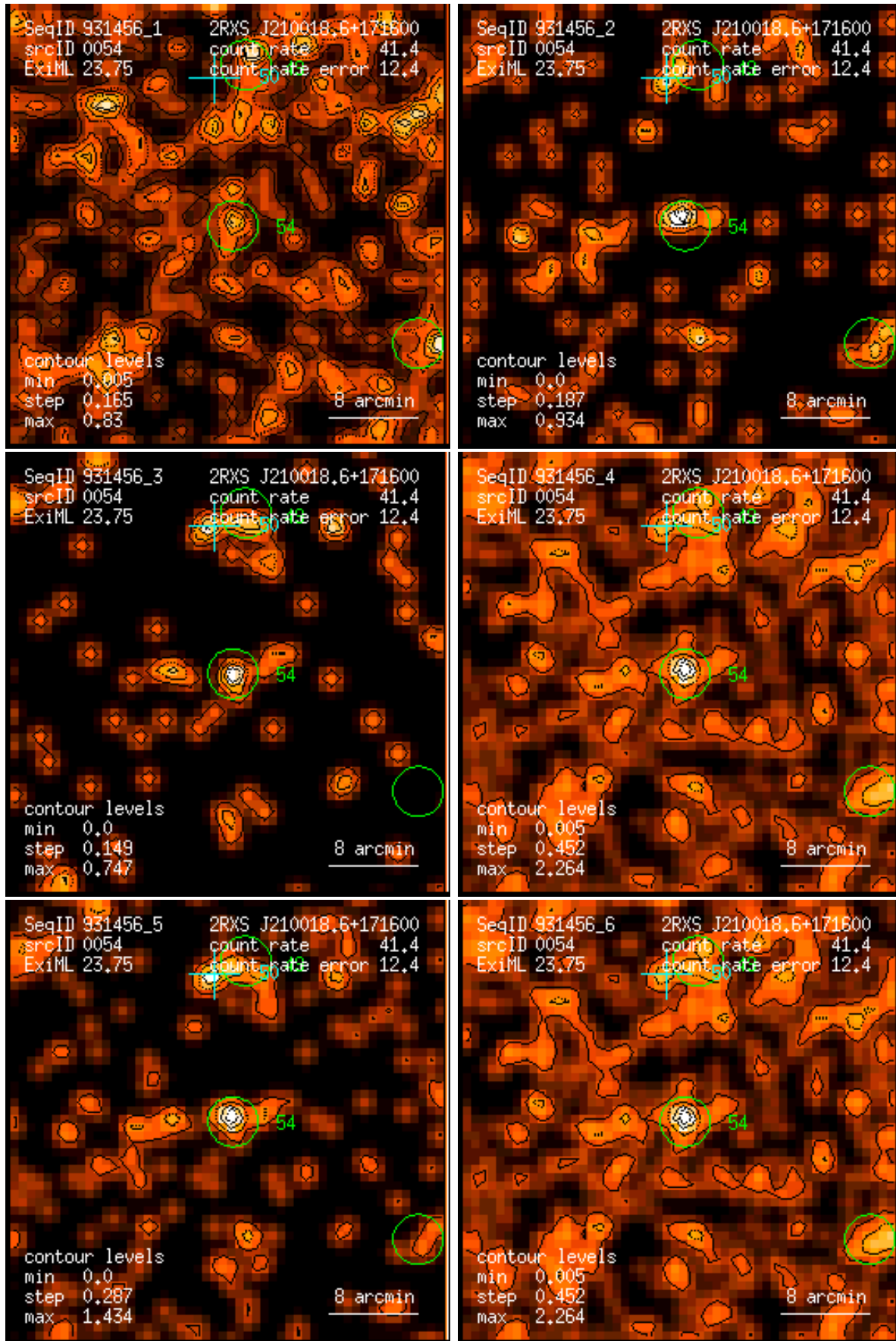
Figure 54: RASS 931456: detection 0054: band rate images, Gaussian filter: (1) PSPC channels 11 – 41, (2) 52 – 90, (3) 91 – 201, (4) 11 – 235, (5) 52 – 201, (6) 11 – 201. Broad band rates in counts/ks. Band rate contour levels in counts/ks/arcmin 2 .
