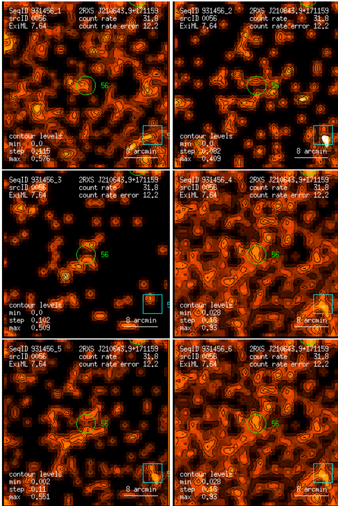
Figure 56: RASS 931456: detection 0056: band rate images, Gaussian filter: (1) PSPC channels 11 – 41, (2) 52 – 90, (3) 91 – 201, (4) 11 – 235, (5) 52 – 201, (6) 11 – 201. Broad band rates in counts/ks. Band rate contour levels in counts/ks/arcmin 2 .
