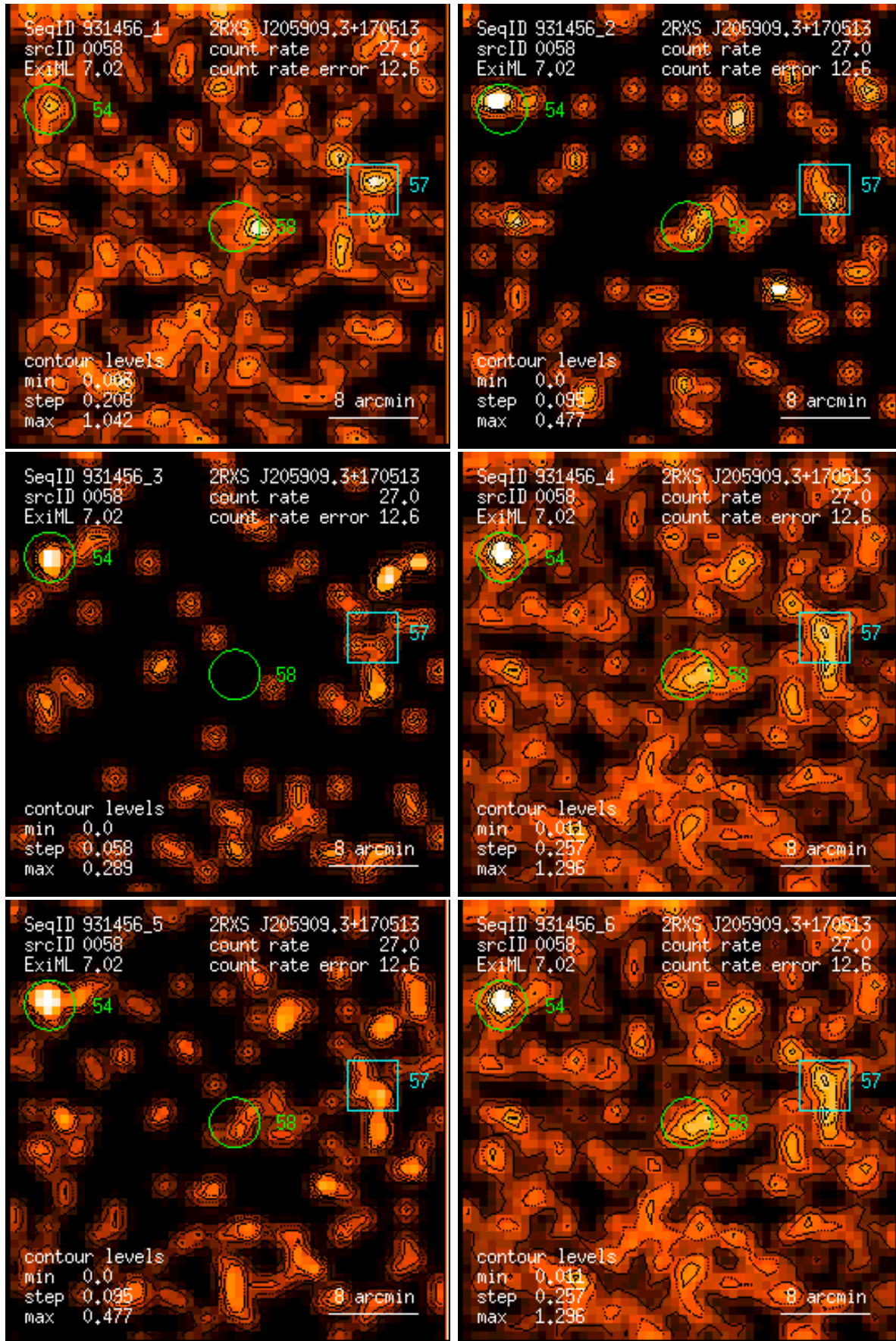
Figure 58: RASS 931456: detection 0058: band rate images, Gaussian filter: (1) PSPC channels 11 – 41, (2) 52 – 90, (3) 91 – 201, (4) 11 – 235, (5) 52 – 201, (6) 11 – 201. Broad band rates in counts/ks. Band rate contour levels in counts/ks/arcmin 2 .
