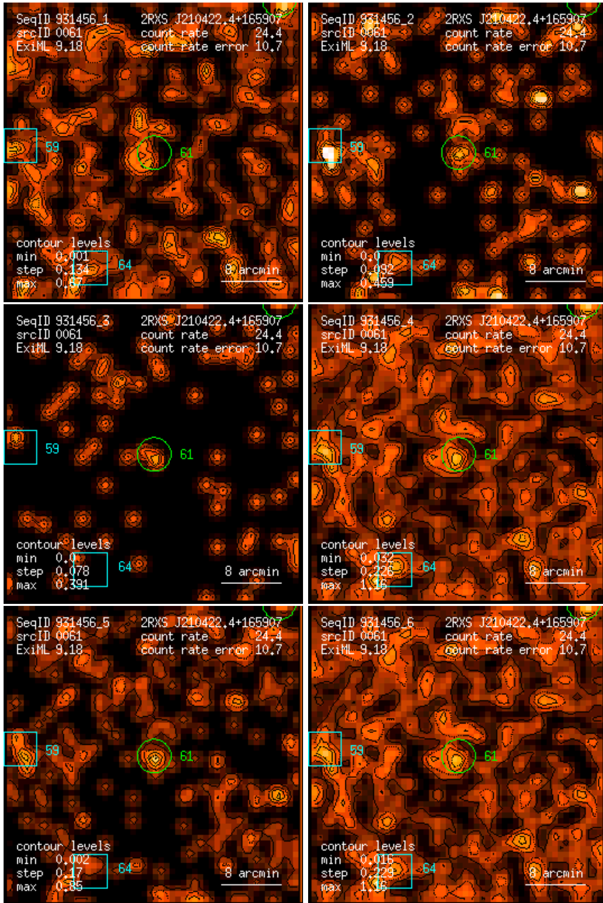
Figure 61: RASS 931456: detection 0061: band rate images, Gaussian filter: (1) PSPC channels 11 – 41, (2) 52 – 90, (3) 91 – 201, (4) 11 – 235, (5) 52 – 201, (6) 11 – 201. Broad band rates in counts/ks. Band rate contour levels in counts/ks/arcmin 2 .
