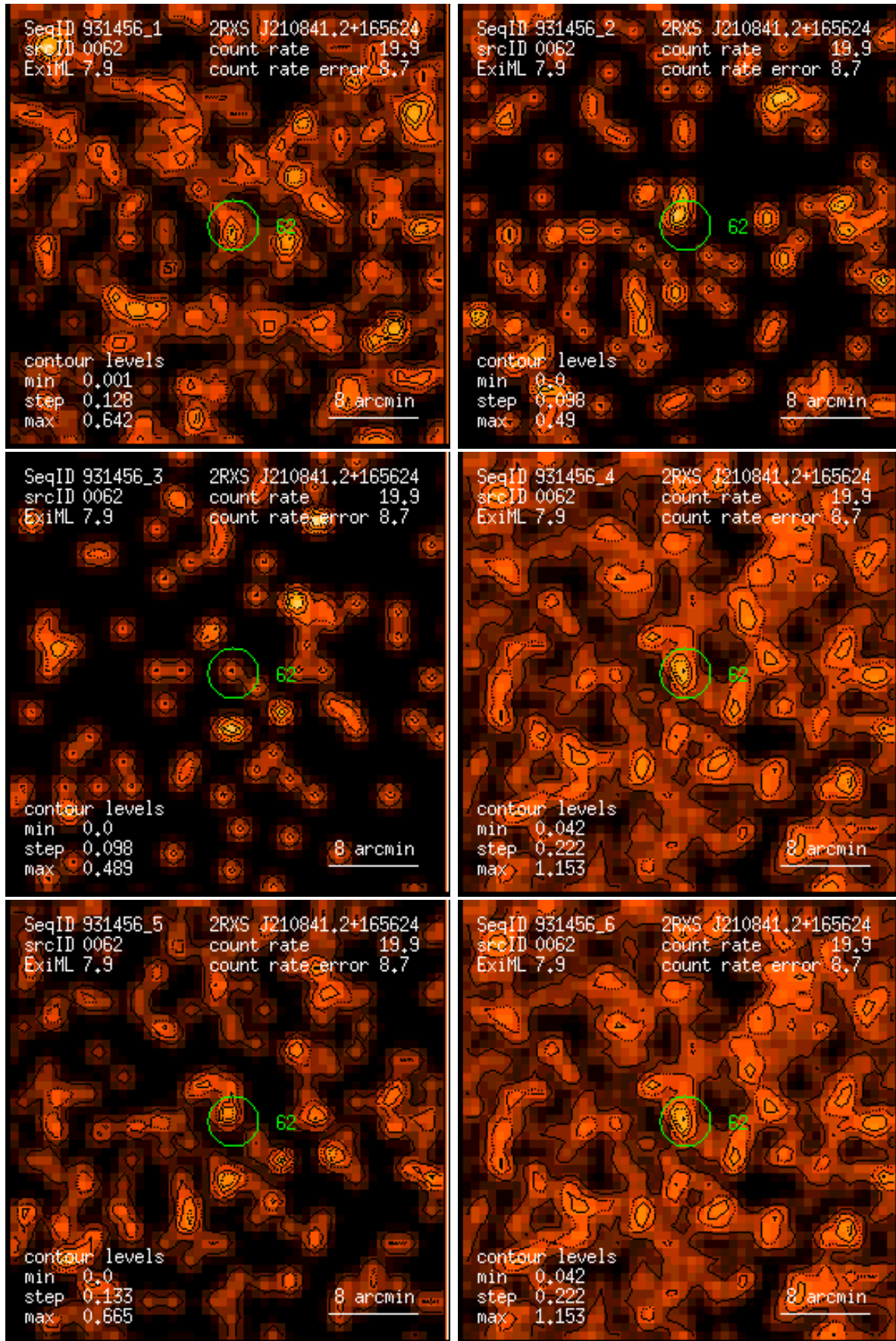
Figure 62: RASS 931456: detection 0062: band rate images, Gaussian filter: (1) PSPC channels 11 – 41, (2) 52 – 90, (3) 91 – 201, (4) 11 – 235, (5) 52 – 201, (6) 11 – 201. Broad band rates in counts/ks. Band rate contour levels in counts/ks/arcmin 2 .
