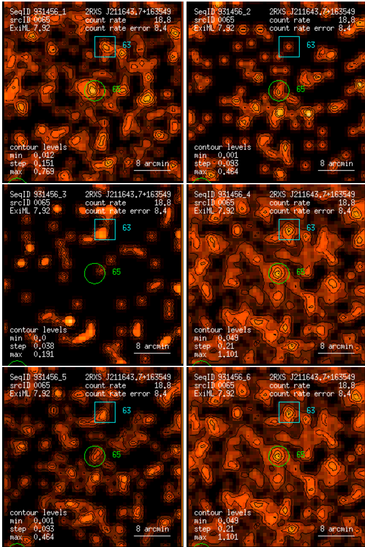
Figure 65: RASS 931456: detection 0065: band rate images, Gaussian filter: (1) PSPC channels 11 – 41, (2) 52 – 90, (3) 91 – 201, (4) 11 – 235, (5) 52 – 201, (6) 11 – 201. Broad band rates in counts/ks. Band rate contour levels in counts/ks/arcmin 2 .
