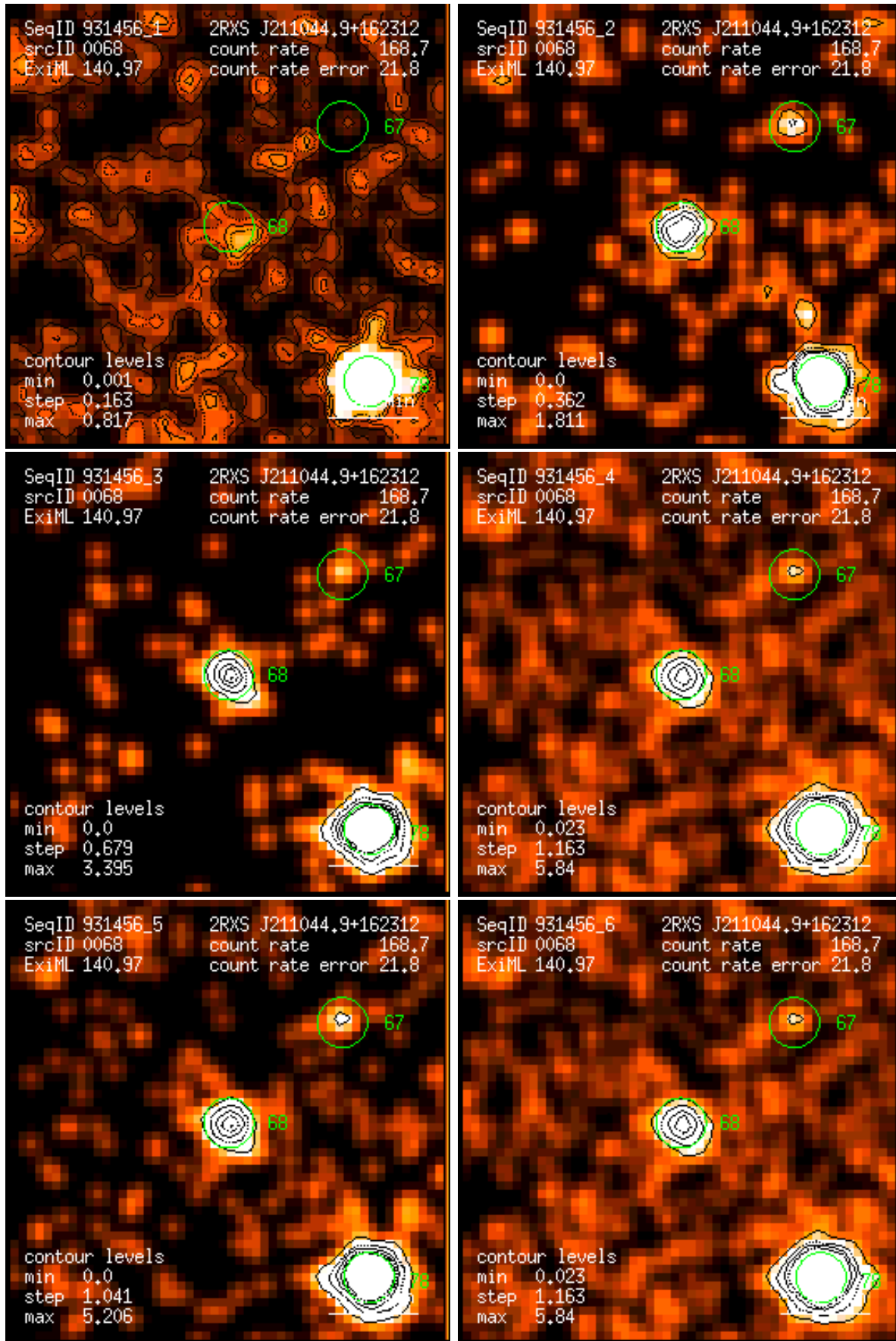
Figure 68: RASS 931456: detection 0068: band rate images, Gaussian filter: (1) PSPC channels 11 – 41, (2) 52 – 90, (3) 91 – 201, (4) 11 – 235, (5) 52 – 201, (6) 11 – 201. Broad band rates in counts/ks. Band rate contour levels in counts/ks/arcmin 2 .
