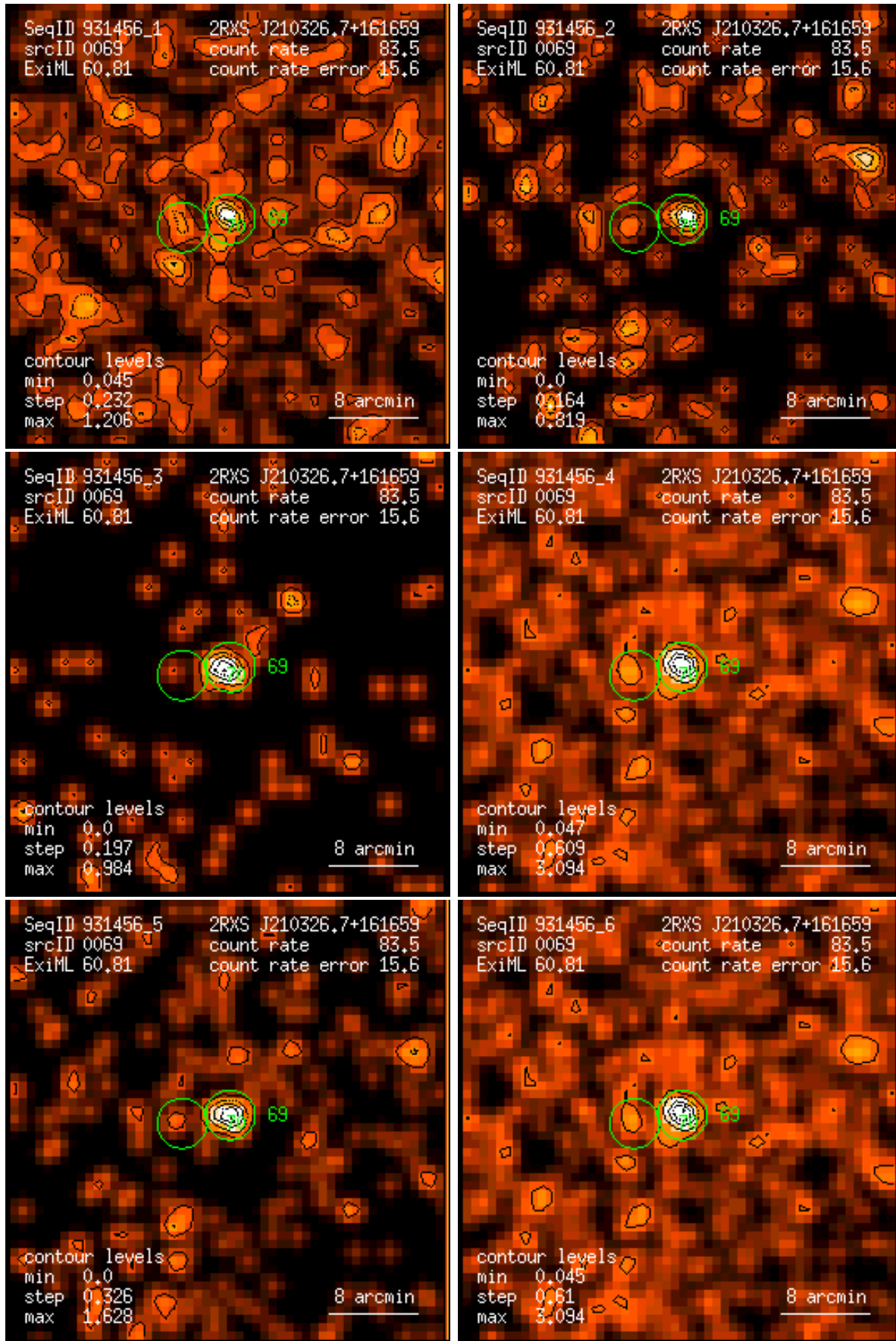
Figure 69: RASS 931456: detection 0069: band rate images, Gaussian filter: (1) PSPC channels 11 – 41, (2) 52 – 90, (3) 91 – 201, (4) 11 – 235, (5) 52 – 201, (6) 11 – 201. Broad band rates in counts/ks. Band rate contour levels in counts/ks/arcmin 2 .
