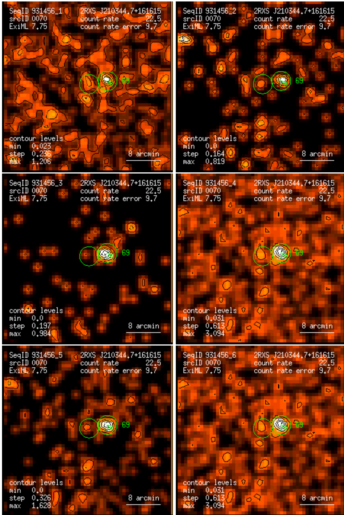
Figure 70: RASS 931456: detection 0070: band rate images, Gaussian filter: (1) PSPC channels 11 – 41, (2) 52 – 90, (3) 91 – 201, (4) 11 – 235, (5) 52 – 201, (6) 11 – 201. Broad band rates in counts/ks. Band rate contour levels in counts/ks/arcmin 2 .
