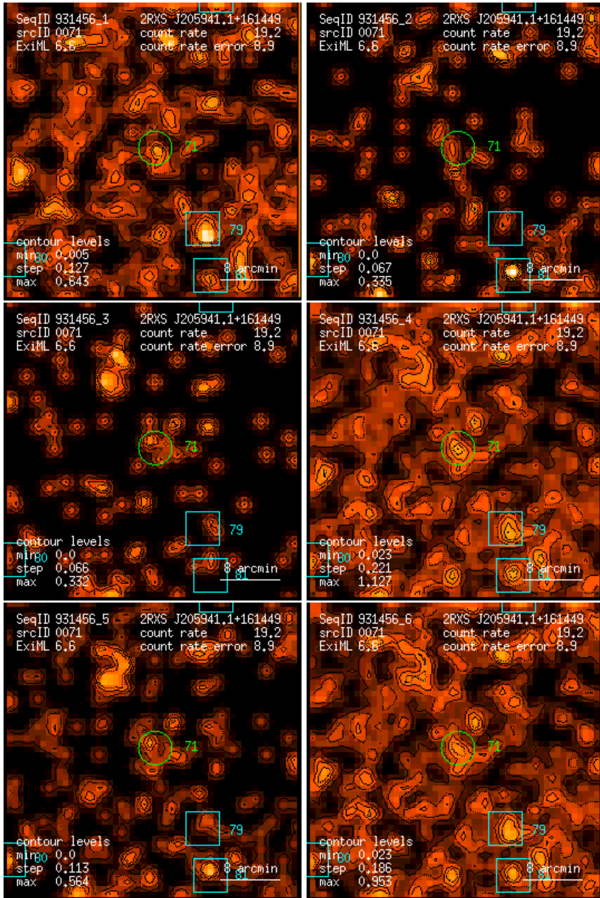
Figure 71: RASS 931456: detection 0071: band rate images, Gaussian filter: (1) PSPC channels 11 – 41, (2) 52 – 90, (3) 91 – 201, (4) 11 – 235, (5) 52 – 201, (6) 11 – 201. Broad band rates in counts/ks. Band rate contour levels in counts/ks/arcmin 2 .
