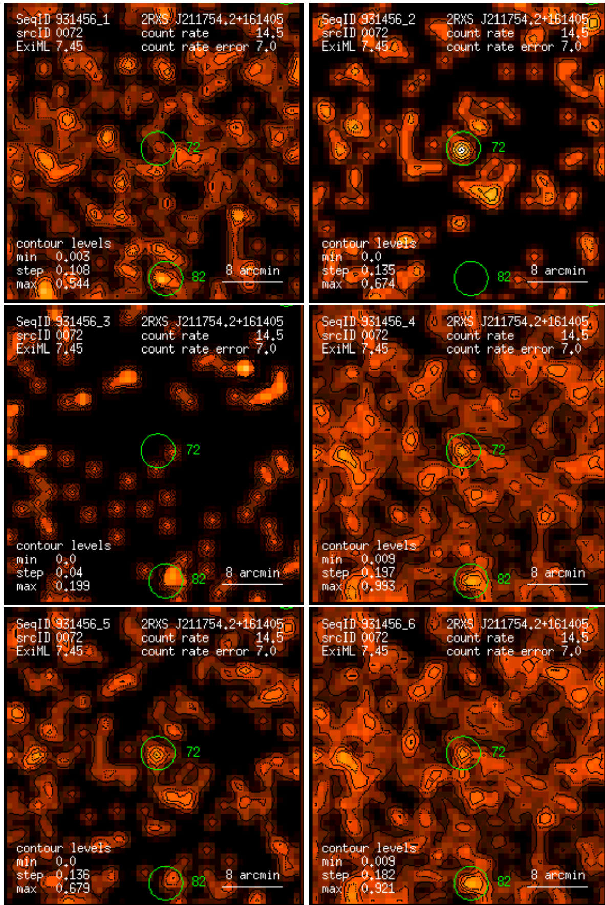
Figure 72: RASS 931456: detection 0072: band rate images, Gaussian filter: (1) PSPC channels 11 – 41, (2) 52 – 90, (3) 91 – 201, (4) 11 – 235, (5) 52 – 201, (6) 11 – 201. Broad band rates in counts/ks. Band rate contour levels in counts/ks/arcmin 2 .
