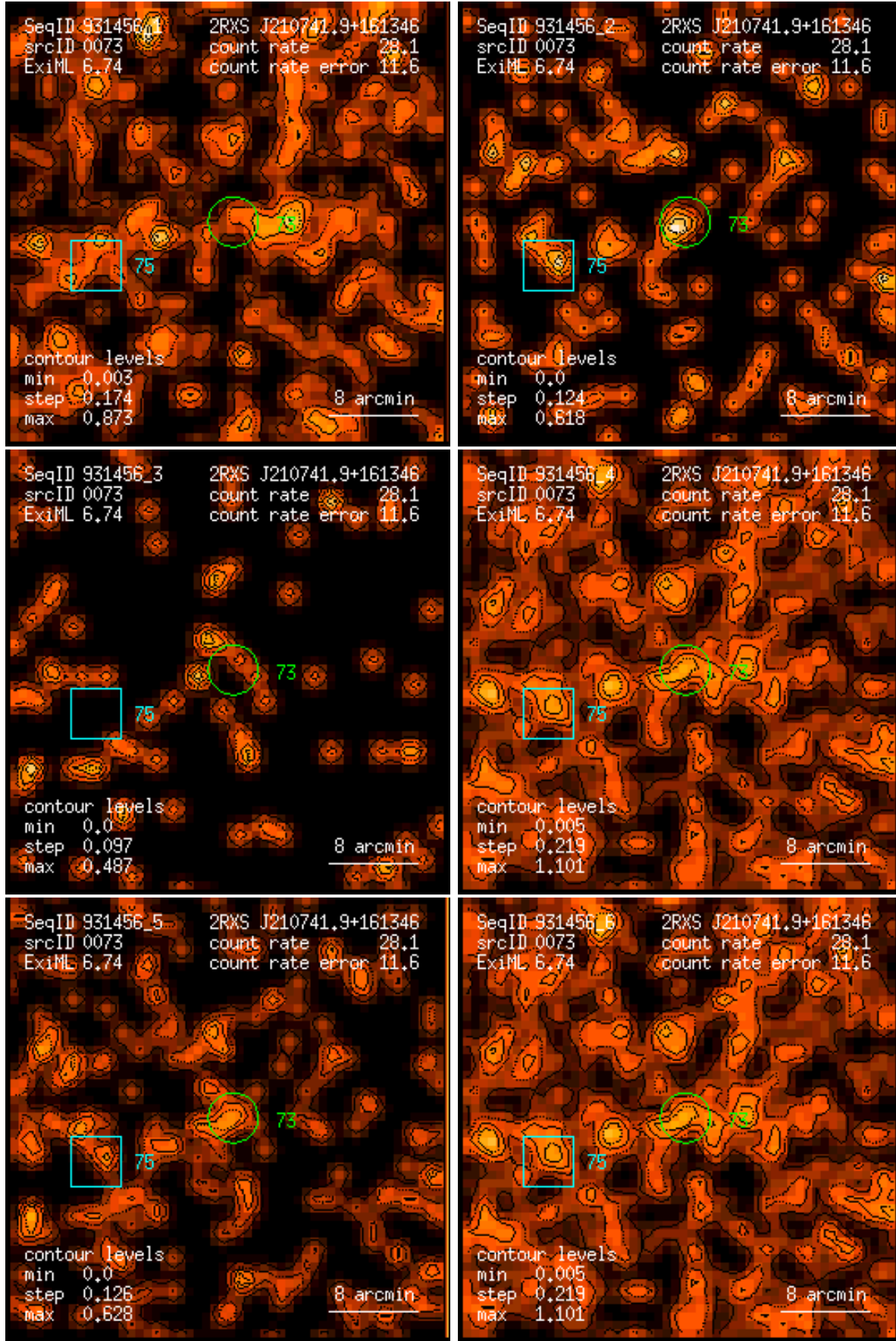
Figure 73: RASS 931456: detection 0073: band rate images, Gaussian filter: (1) PSPC channels 11 – 41, (2) 52 – 90, (3) 91 – 201, (4) 11 – 235, (5) 52 – 201, (6) 11 – 201. Broad band rates in counts/ks. Band rate contour levels in counts/ks/arcmin 2 .
