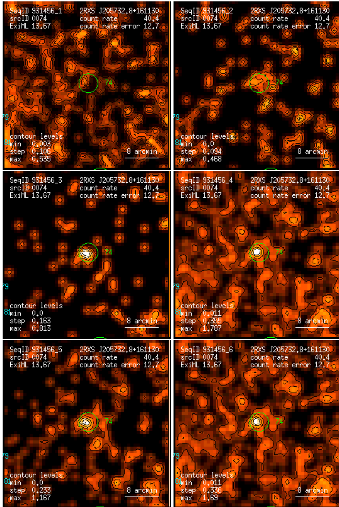
Figure 74: RASS 931456: detection 0074: band rate images, Gaussian filter: (1) PSPC channels 11 – 41, (2) 52 – 90, (3) 91 – 201, (4) 11 – 235, (5) 52 – 201, (6) 11 – 201. Broad band rates in counts/ks. Band rate contour levels in counts/ks/arcmin 2 .
