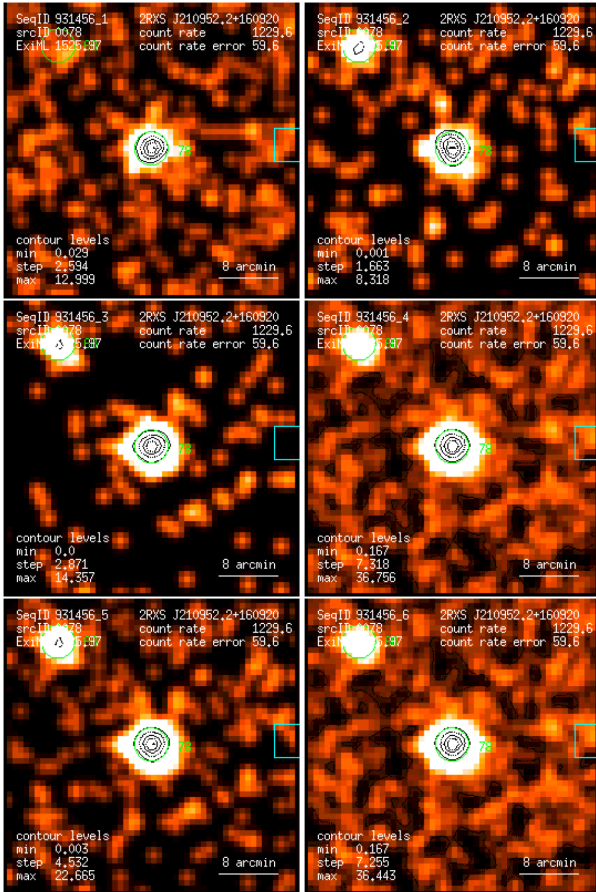
Figure 78: RASS 931456: detection 0078: band rate images, Gaussian filter: (1) PSPC channels 11 – 41, (2) 52 – 90, (3) 91 – 201, (4) 11 – 235, (5) 52 – 201, (6) 11 – 201. Broad band rates in counts/ks. Band rate contour levels in counts/ks/arcmin 2 .
