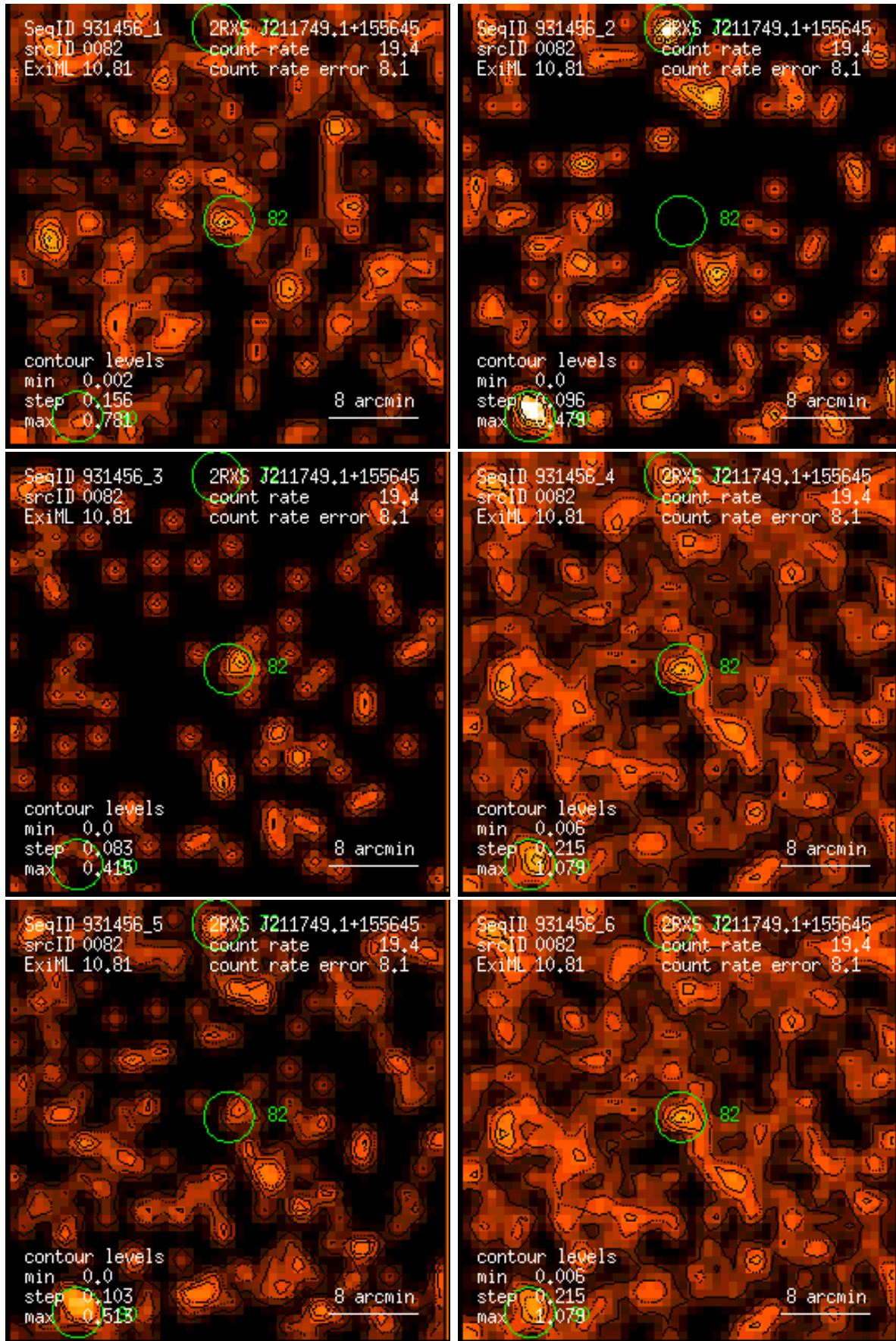
Figure 82: RASS 931456: detection 0082: band rate images, Gaussian filter: (1) PSPC channels 11 – 41, (2) 52 – 90, (3) 91 – 201, (4) 11 – 235, (5) 52 – 201, (6) 11 – 201. Broad band rates in counts/ks. Band rate contour levels in counts/ks/arcmin 2 .
