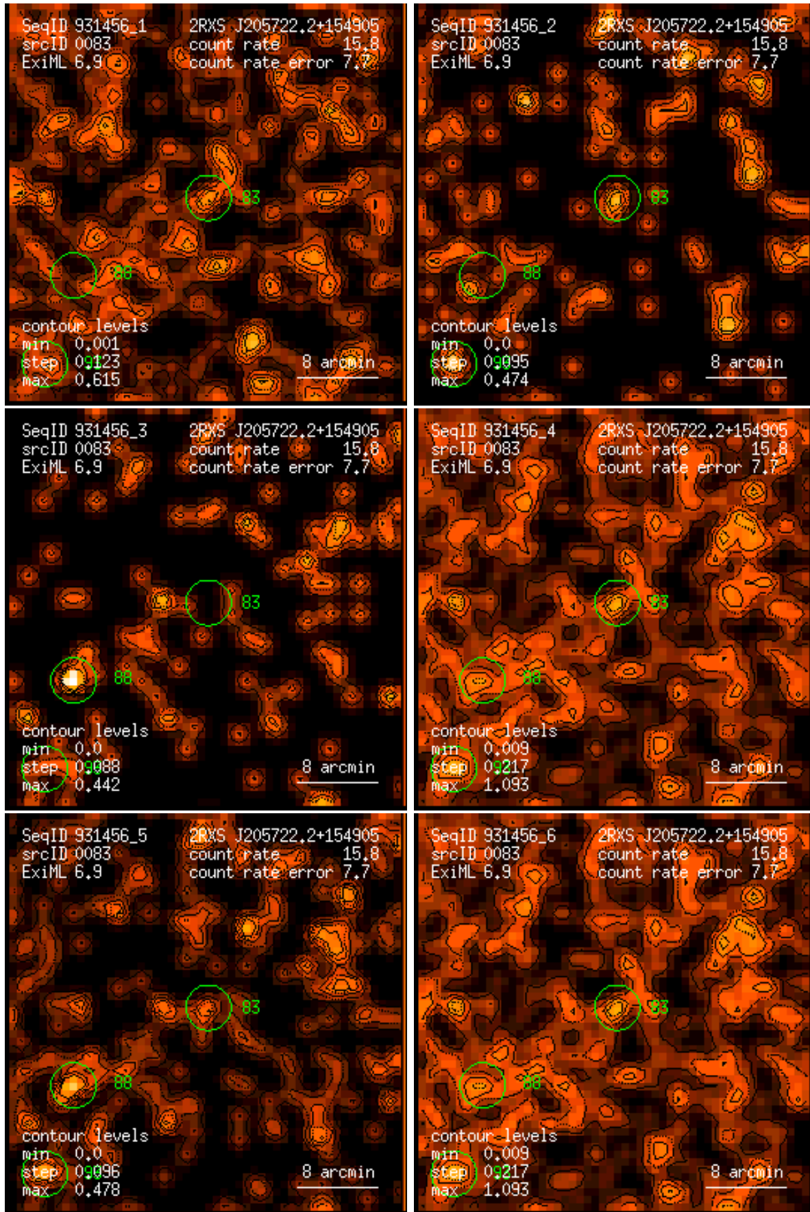
Figure 83: RASS 931456: detection 0083: band rate images, Gaussian filter: (1) PSPC channels 11 – 41, (2) 52 – 90, (3) 91 – 201, (4) 11 – 235, (5) 52 – 201, (6) 11 – 201. Broad band rates in counts/ks. Band rate contour levels in counts/ks/arcmin 2 .
