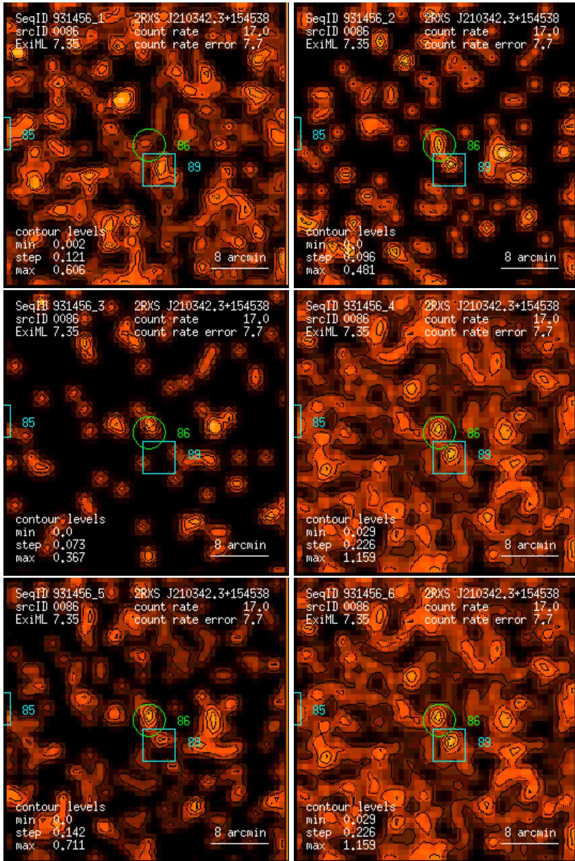
Figure 86: RASS 931456: detection 0086: band rate images, Gaussian filter: (1) PSPC channels 11 – 41, (2) 52 – 90, (3) 91 – 201, (4) 11 – 235, (5) 52 – 201, (6) 11 – 201. Broad band rates in counts/ks. Band rate contour levels in counts/ks/arcmin 2 .
