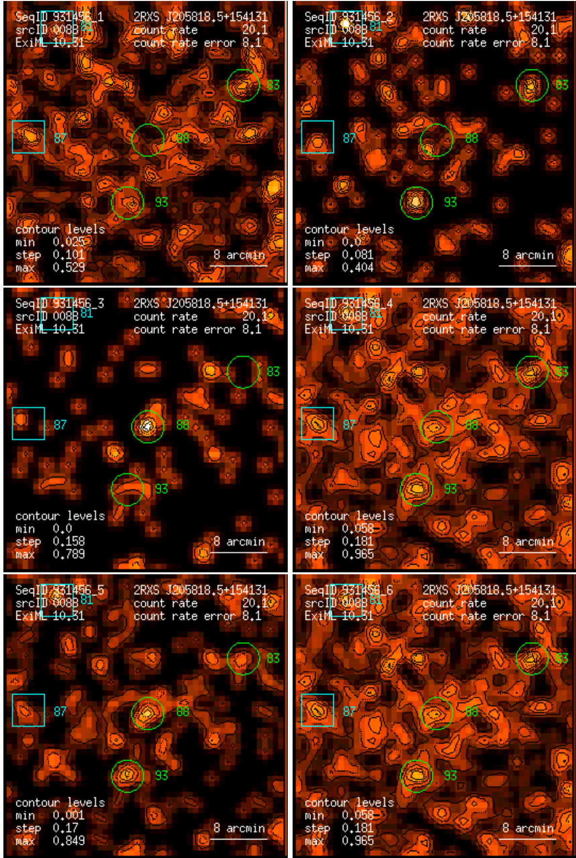
Figure 88: RASS 931456: detection 0088: band rate images, Gaussian filter: (1) PSPC channels 11 – 41, (2) 52 – 90, (3) 91 – 201, (4) 11 – 235, (5) 52 – 201, (6) 11 – 201. Broad band rates in counts/ks. Band rate contour levels in counts/ks/arcmin 2 .
