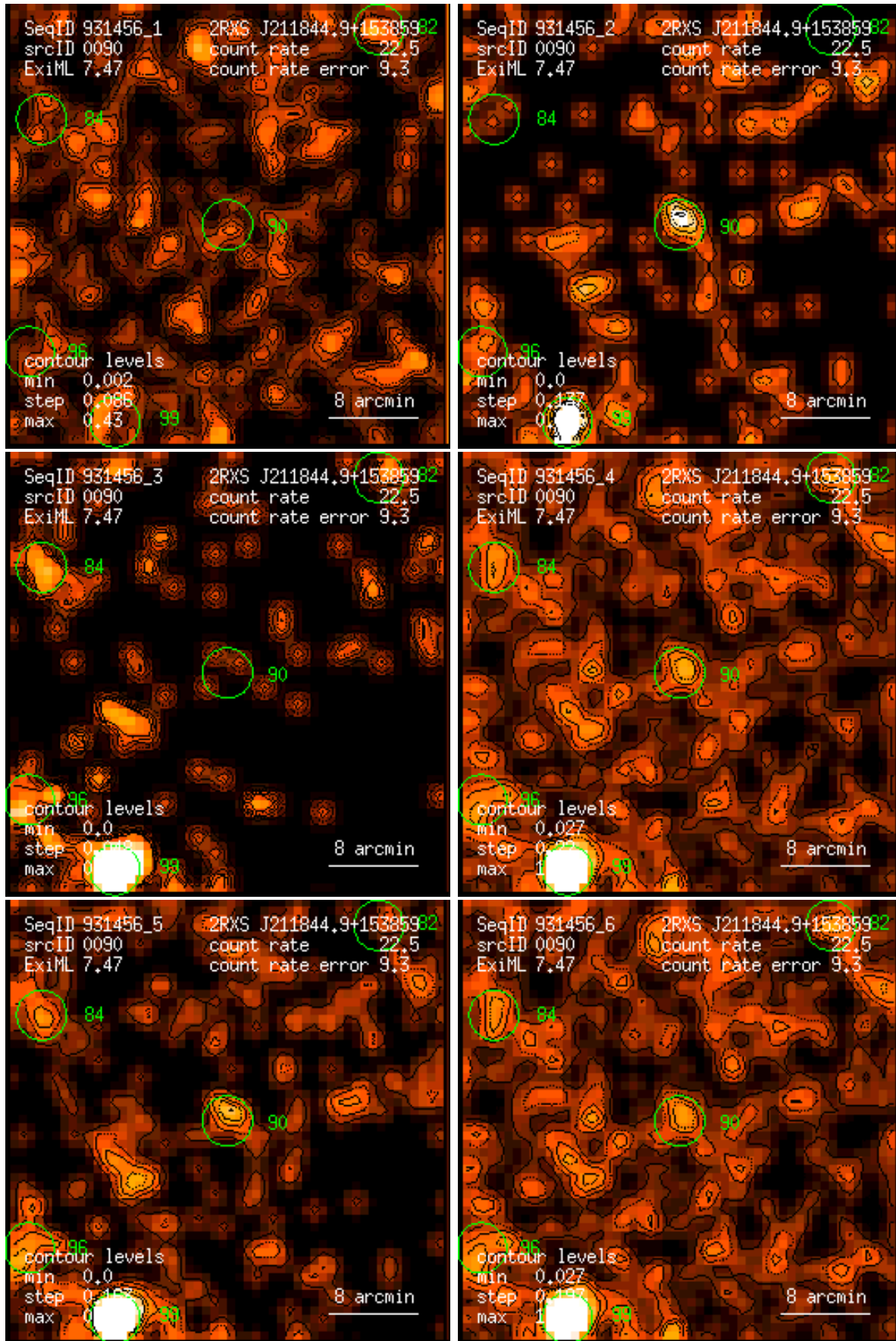
Figure 90: RASS 931456: detection 0090: band rate images, Gaussian filter: (1) PSPC channels 11 – 41, (2) 52 – 90, (3) 91 – 201, (4) 11 – 235, (5) 52 – 201, (6) 11 – 201. Broad band rates in counts/ks. Band rate contour levels in counts/ks/arcmin 2 .
