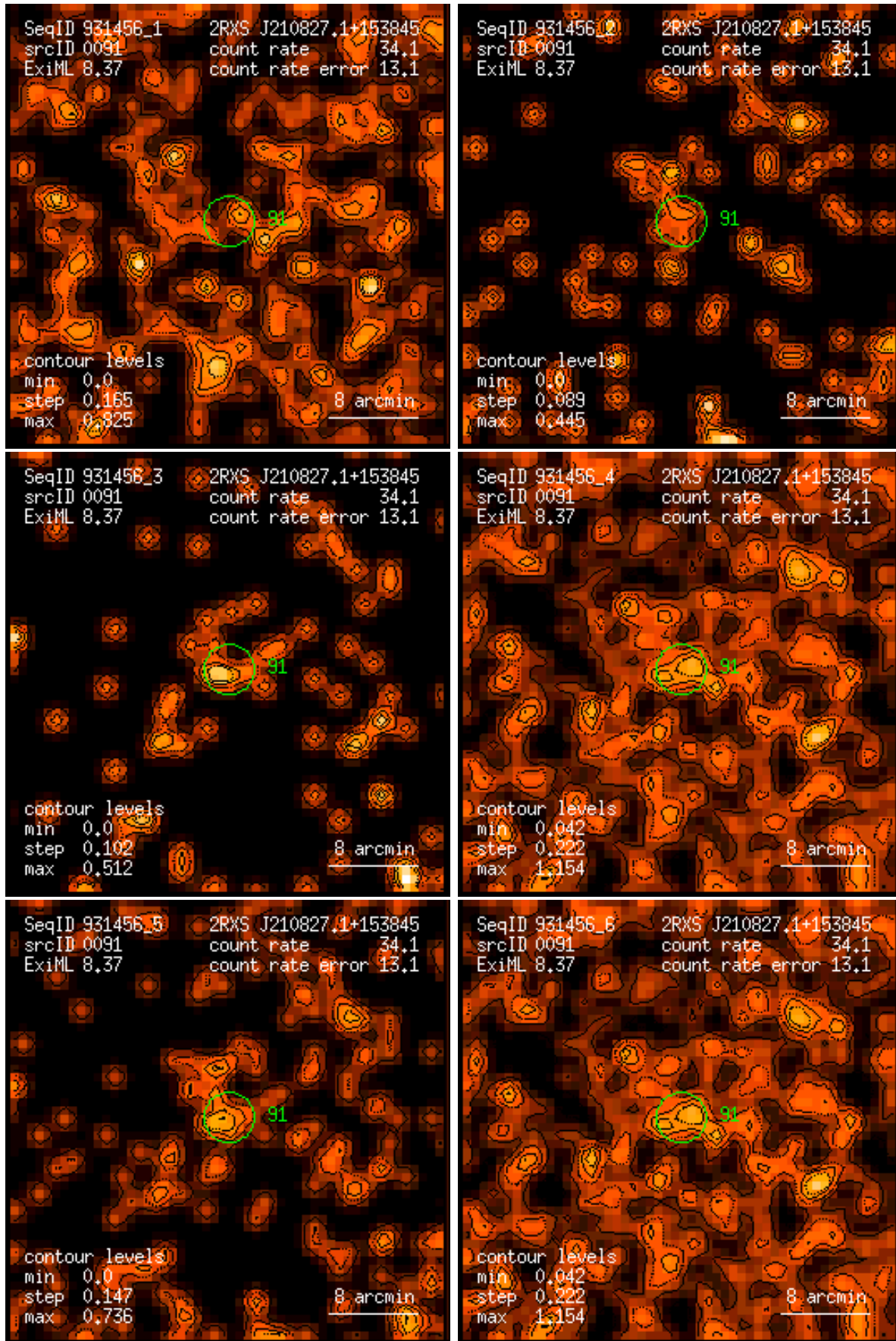
Figure 91: RASS 931456: detection 0091: band rate images, Gaussian filter: (1) PSPC channels 11 – 41, (2) 52 – 90, (3) 91 – 201, (4) 11 – 235, (5) 52 – 201, (6) 11 – 201. Broad band rates in counts/ks. Band rate contour levels in counts/ks/arcmin 2 .
