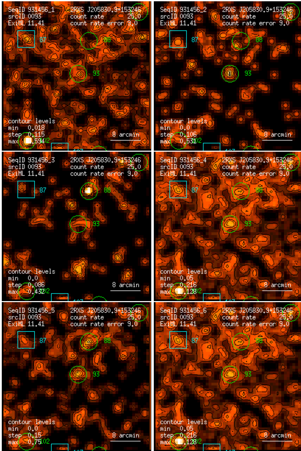
Figure 93: RASS 931456: detection 0093: band rate images, Gaussian filter: (1) PSPC channels 11 – 41, (2) 52 – 90, (3) 91 – 201, (4) 11 – 235, (5) 52 – 201, (6) 11 – 201. Broad band rates in counts/ks. Band rate contour levels in counts/ks/arcmin 2 .
